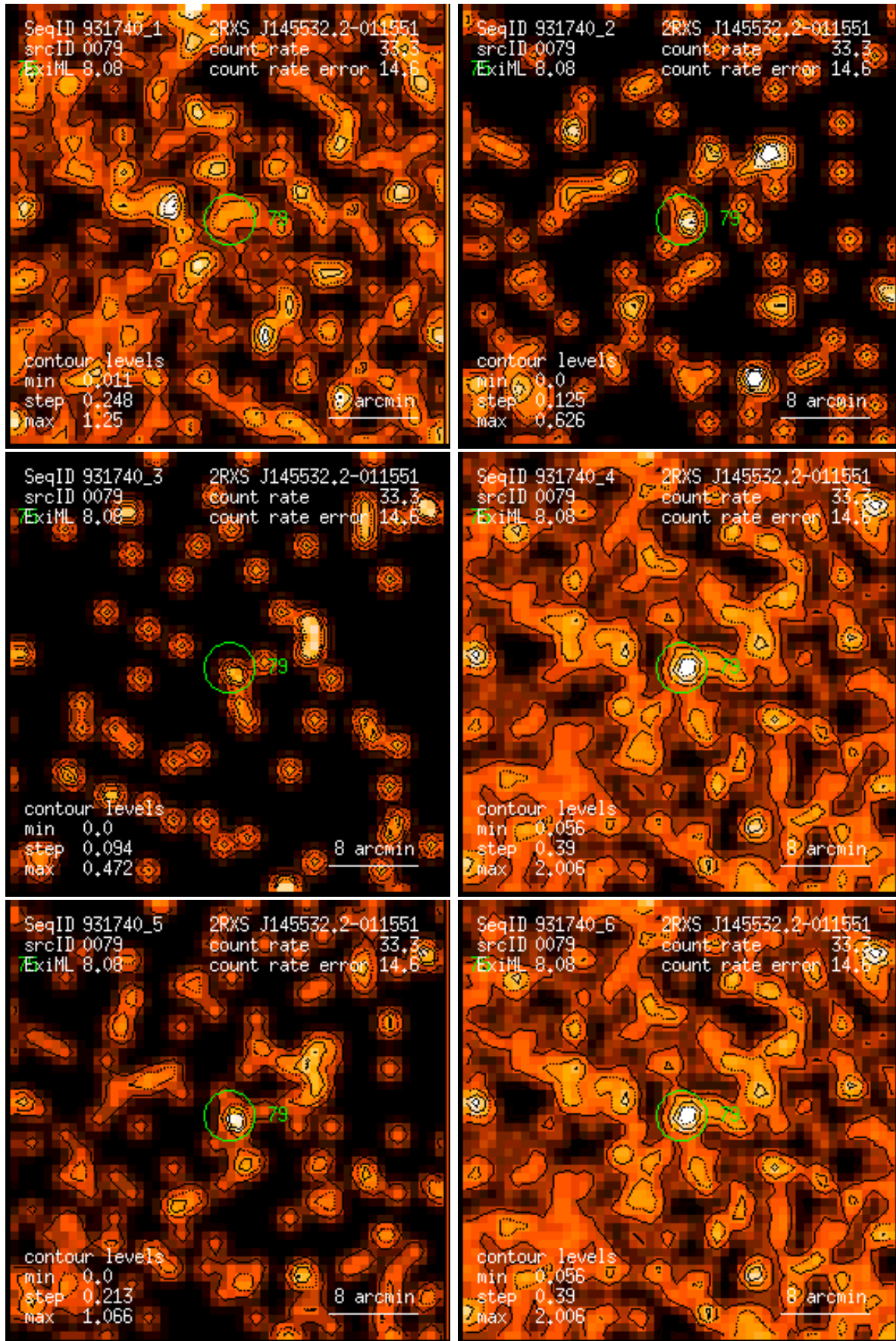
Figure 79: RASS 931740: detection 0079: band rate images, Gaussian filter: (1) PSPC channels 11 – 41, (2) 52 – 90, (3) 91 – 201, (4) 11 – 235, (5) 52 – 201, (6) 11 – 201. Broad band rates in counts/ks. Band rate contour levels in counts/ks/arcmin 2 .
