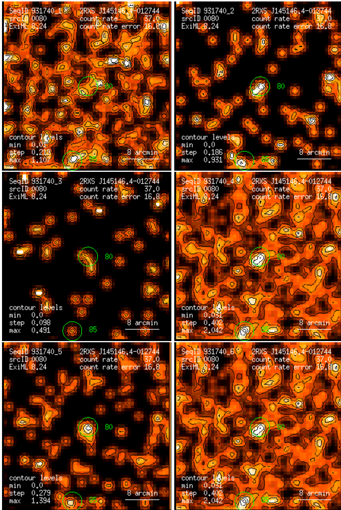
Figure 80: RASS 931740: detection 0080: band rate images, Gaussian filter: (1) PSPC channels 11 – 41, (2) 52 – 90, (3) 91 – 201, (4) 11 – 235, (5) 52 – 201, (6) 11 – 201. Broad band rates in counts/ks. Band rate contour levels in counts/ks/arcmin 2 .
