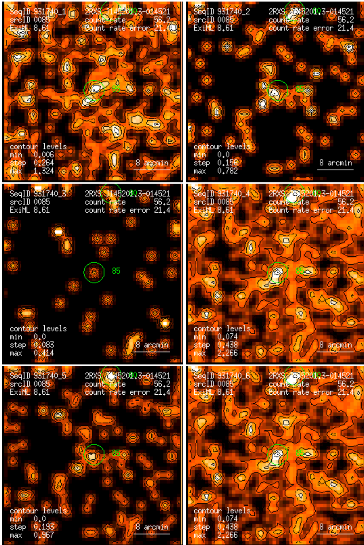
Figure 85: RASS 931740: detection 0085: band rate images, Gaussian filter: (1) PSPC channels 11 – 41, (2) 52 – 90, (3) 91 – 201, (4) 11 – 235, (5) 52 – 201, (6) 11 – 201. Broad band rates in counts/ks. Band rate contour levels in counts/ks/arcmin 2 .
