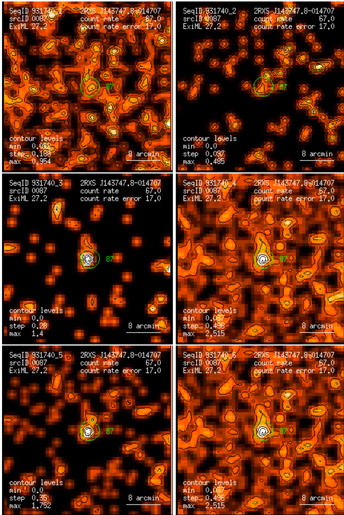
Figure 87: RASS 931740: detection 0087: band rate images, Gaussian filter: (1) PSPC channels 11 – 41, (2) 52 – 90, (3) 91 – 201, (4) 11 – 235, (5) 52 – 201, (6) 11 – 201. Broad band rates in counts/ks. Band rate contour levels in counts/ks/arcmin 2 .
