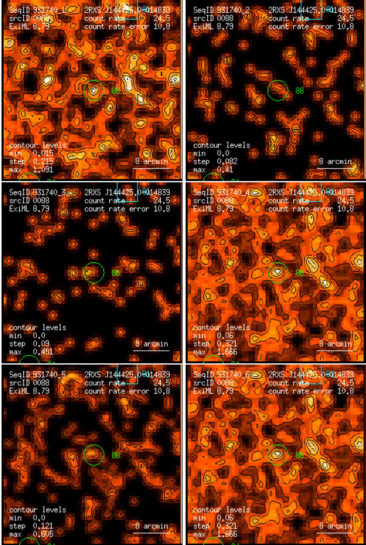
Figure 88: RASS 931740: detection 0088: band rate images, Gaussian filter: (1) PSPC channels 11 – 41, (2) 52 – 90, (3) 91 – 201, (4) 11 – 235, (5) 52 – 201, (6) 11 – 201. Broad band rates in counts/ks. Band rate contour levels in counts/ks/arcmin 2 .
