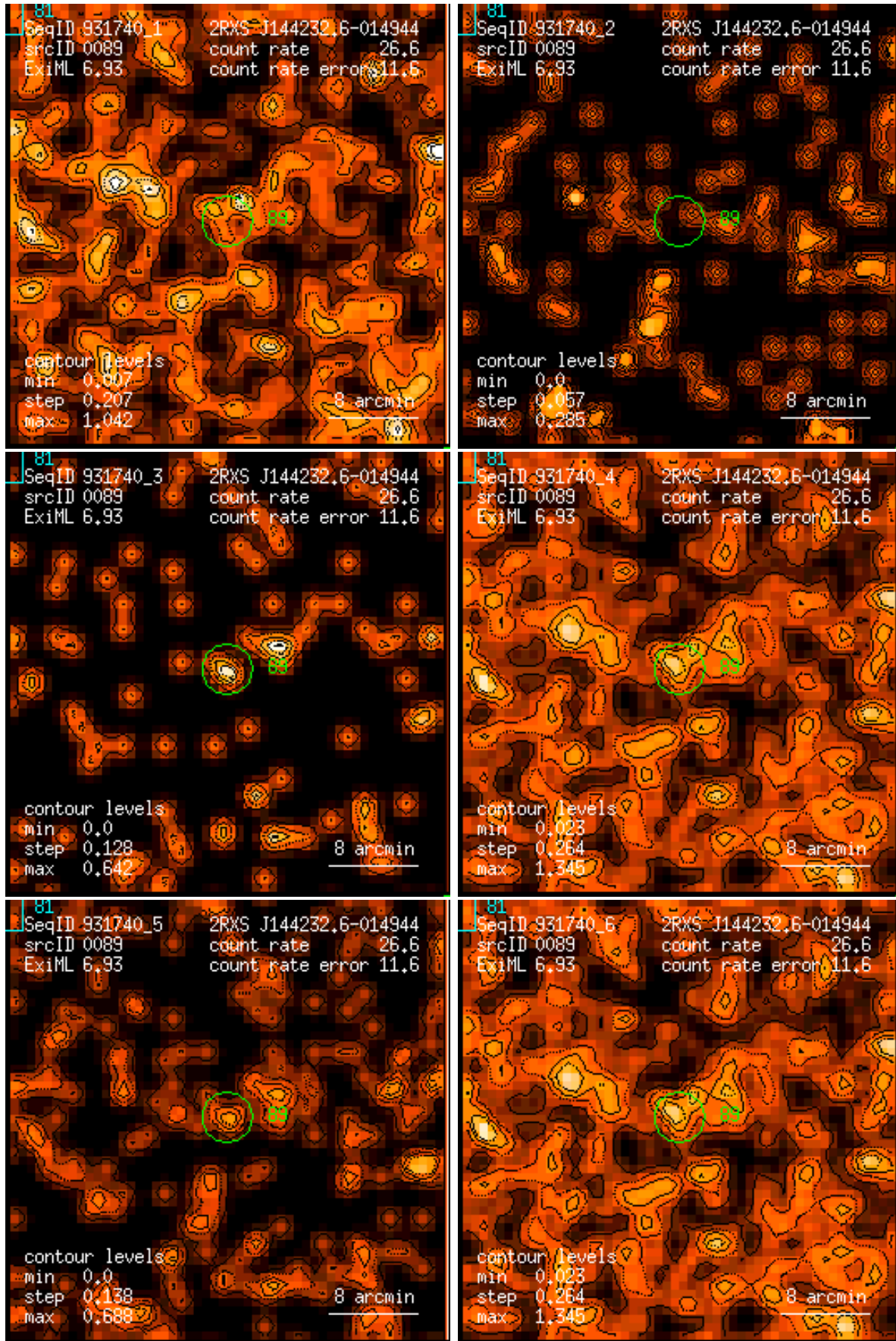
Figure 89: RASS 931740: detection 0089: band rate images, Gaussian filter: (1) PSPC channels 11 – 41, (2) 52 – 90, (3) 91 – 201, (4) 11 – 235, (5) 52 – 201, (6) 11 – 201. Broad band rates in counts/ks. Band rate contour levels in counts/ks/arcmin 2 .
