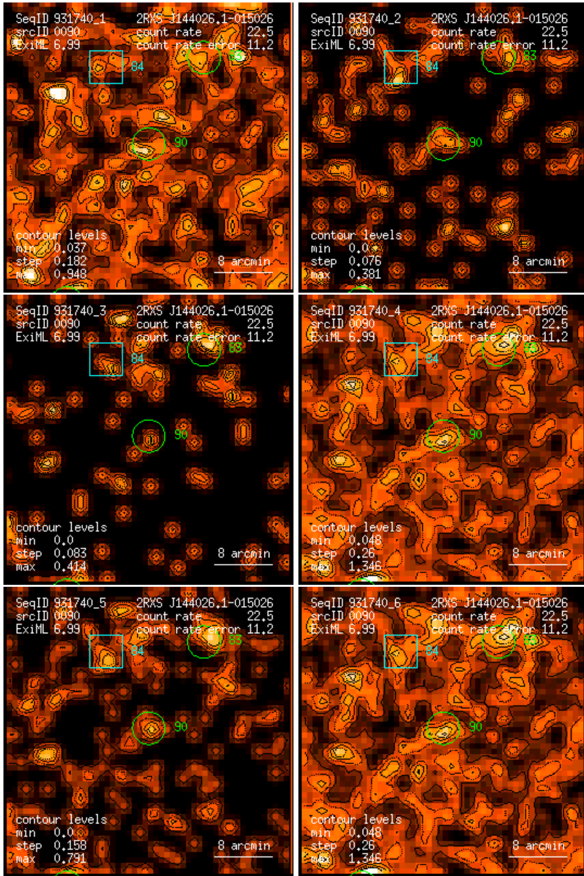
Figure 90: RASS 931740: detection 0090: band rate images, Gaussian filter: (1) PSPC channels 11 – 41, (2) 52 – 90, (3) 91 – 201, (4) 11 – 235, (5) 52 – 201, (6) 11 – 201. Broad band rates in counts/ks. Band rate contour levels in counts/ks/arcmin 2 .
