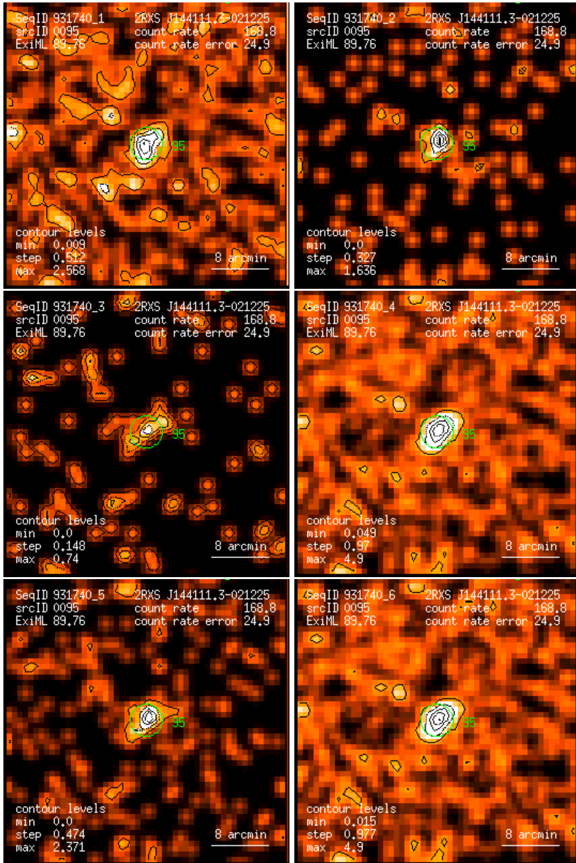
Figure 95: RASS 931740: detection 0095: band rate images, Gaussian filter: (1) PSPC channels 11 – 41, (2) 52 – 90, (3) 91 – 201, (4) 11 – 235, (5) 52 – 201, (6) 11 – 201. Broad band rates in counts/ks. Band rate contour levels in counts/ks/arcmin 2 .
