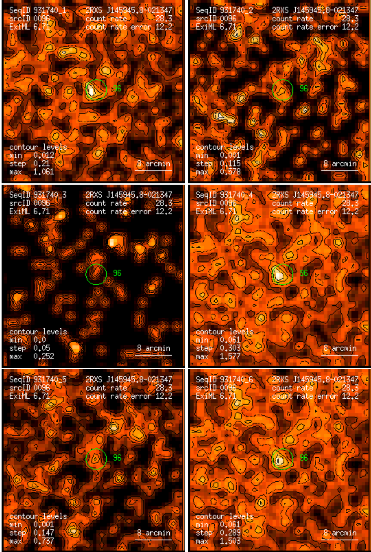
Figure 96: RASS 931740: detection 0096: band rate images, Gaussian filter: (1) PSPC channels 11 – 41, (2) 52 – 90, (3) 91 – 201, (4) 11 – 235, (5) 52 – 201, (6) 11 – 201. Broad band rates in counts/ks. Band rate contour levels in counts/ks/arcmin 2 .
