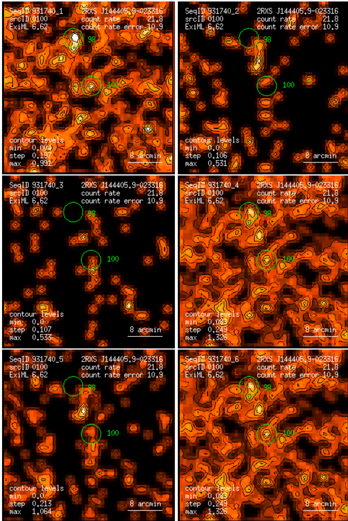
Figure 100: RASS 931740: detection 0100: band rate images, Gaussian filter: (1) PSPC channels 11 – 41, (2) 52 – 90, (3) 91 – 201, (4) 11 – 235, (5) 52 – 201, (6) 11 – 201. Broad band rates in counts/ks. Band rate contour levels in counts/ks/arcmin 2 .
