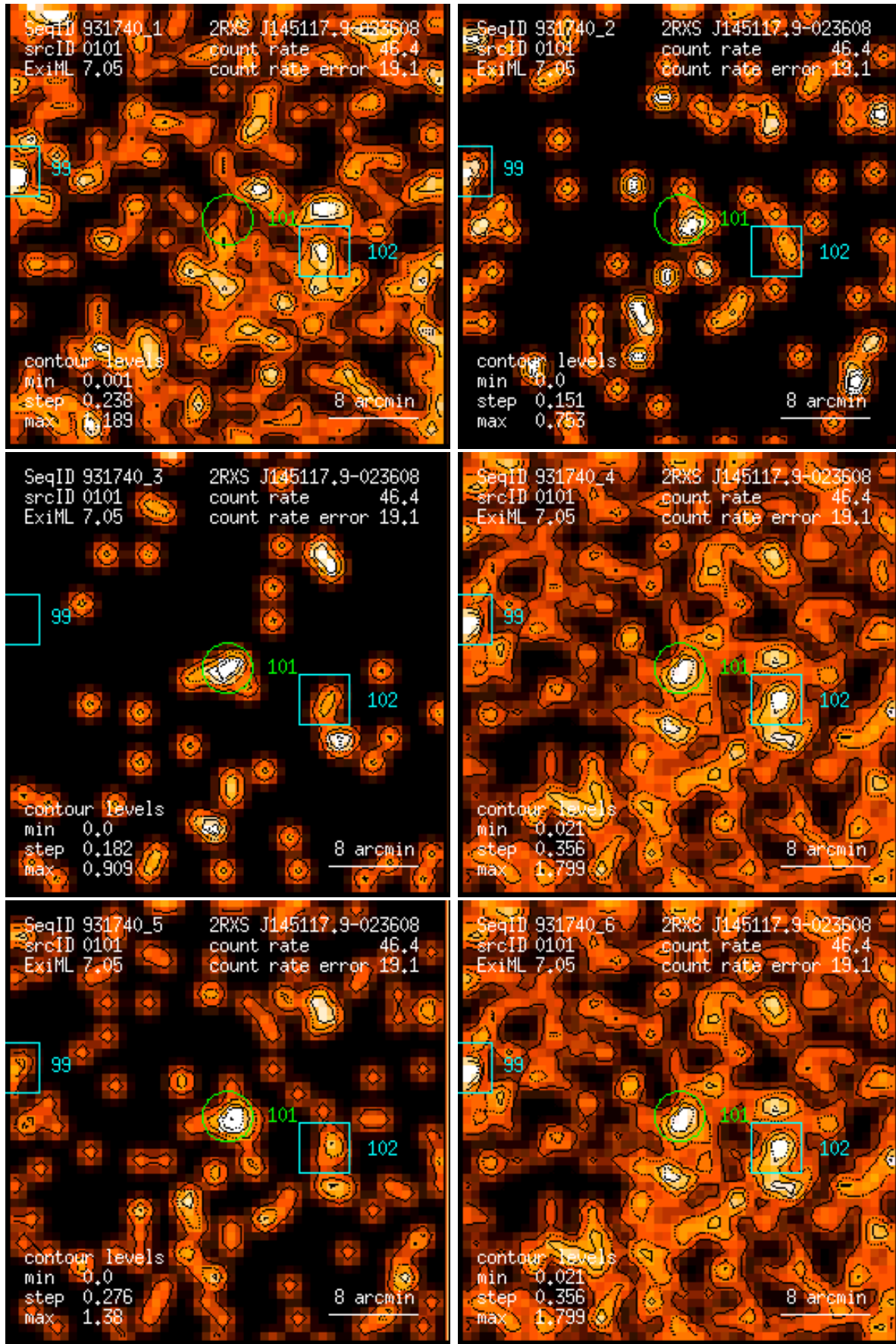
Figure 101: RASS 931740: detection 0101: band rate images, Gaussian filter: (1) PSPC channels 11 – 41, (2) 52 – 90, (3) 91 – 201, (4) 11 – 235, (5) 52 – 201, (6) 11 – 201. Broad band rates in counts/ks. Band rate contour levels in counts/ks/arcmin 2 .
