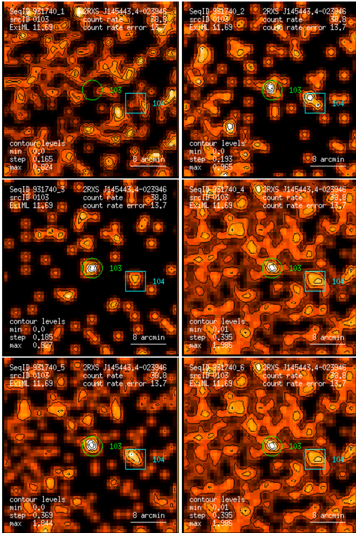
Figure 103: RASS 931740: detection 0103: band rate images, Gaussian filter: (1) PSPC channels 11 – 41, (2) 52 – 90, (3) 91 – 201, (4) 11 – 235, (5) 52 – 201, (6) 11 – 201. Broad band rates in counts/ks. Band rate contour levels in counts/ks/arcmin 2 .
