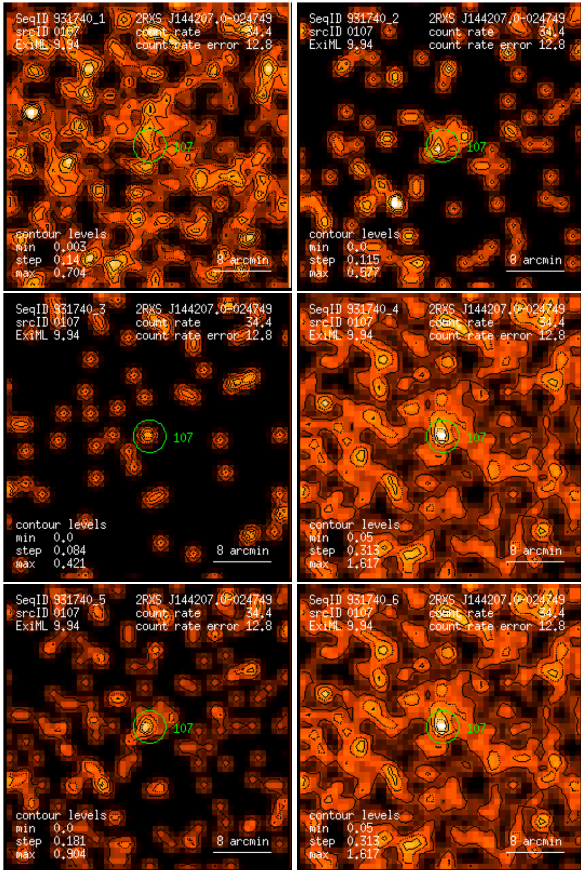
Figure 107: RASS 931740: detection 0107: band rate images, Gaussian filter: (1) PSPC channels 11 – 41, (2) 52 – 90, (3) 91 – 201, (4) 11 – 235, (5) 52 – 201, (6) 11 – 201. Broad band rates in counts/ks. Band rate contour levels in counts/ks/arcmin 2 .
