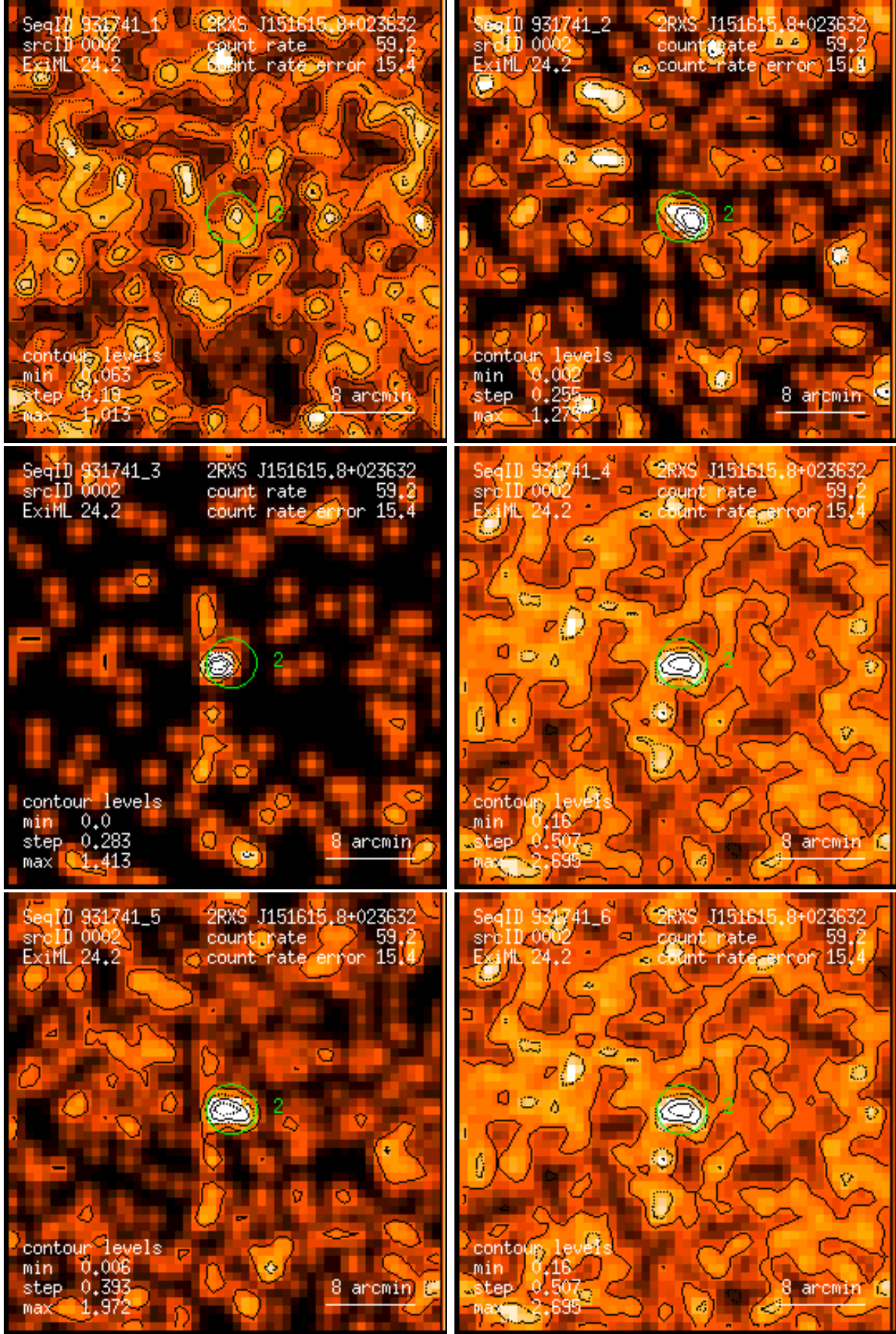
Figure 2: RASS 931741: detection 0002: band rate images, Gaussian filter: (1) PSPC channels 11 – 41, (2) 52 – 90, (3) 91 – 201, (4) 11 – 235, (5) 52 – 201, (6) 11 – 201. Broad band rates in counts/ks. Band rate contour levels in counts/ks/arcmin 2 .
