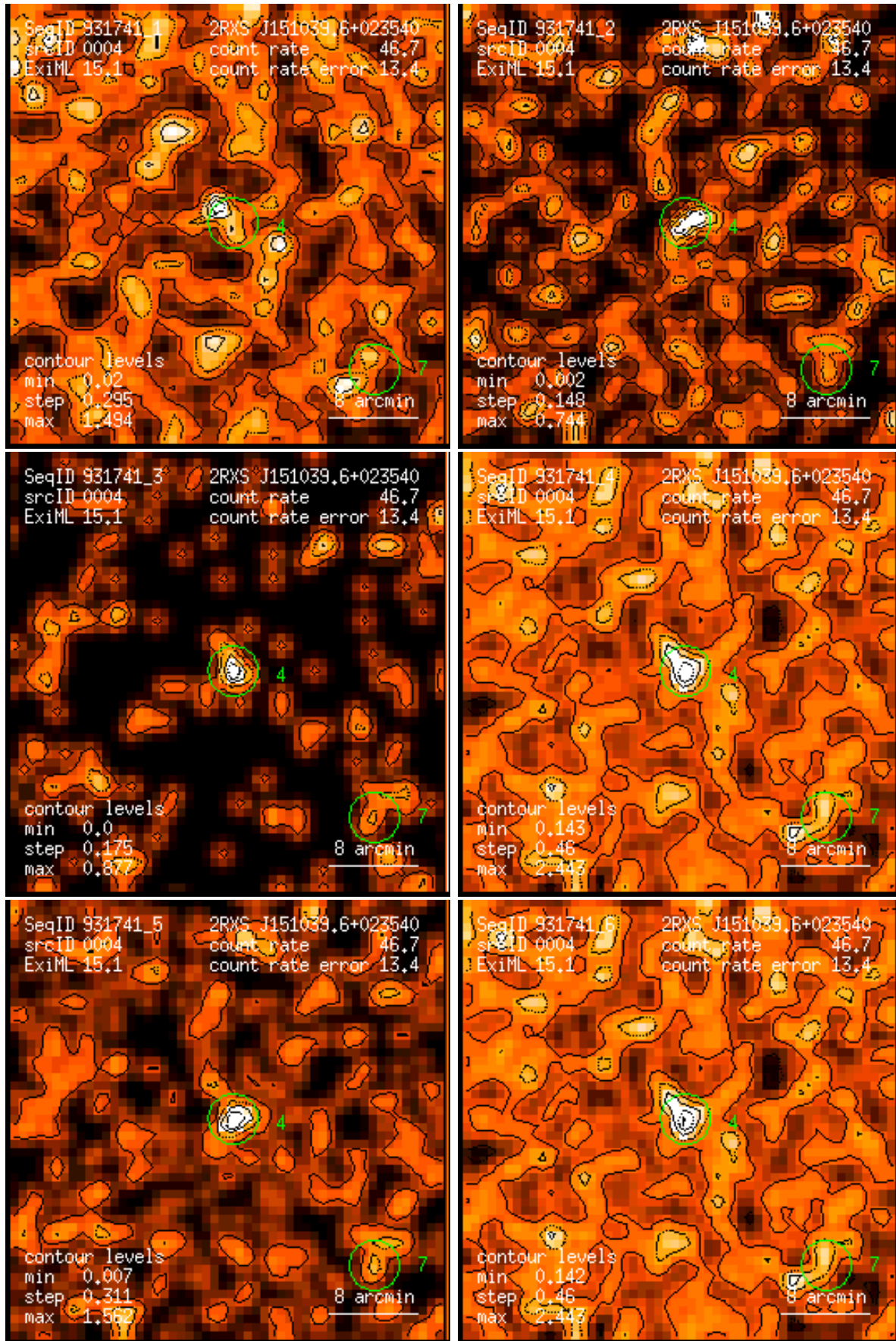
Figure 4: RASS 931741: detection 0004: band rate images, Gaussian filter: (1) PSPC channels 11 – 41, (2) 52 – 90, (3) 91 – 201, (4) 11 – 235, (5) 52 – 201, (6) 11 – 201. Broad band rates in counts/ks. Band rate contour levels in counts/ks/arcmin 2 .
