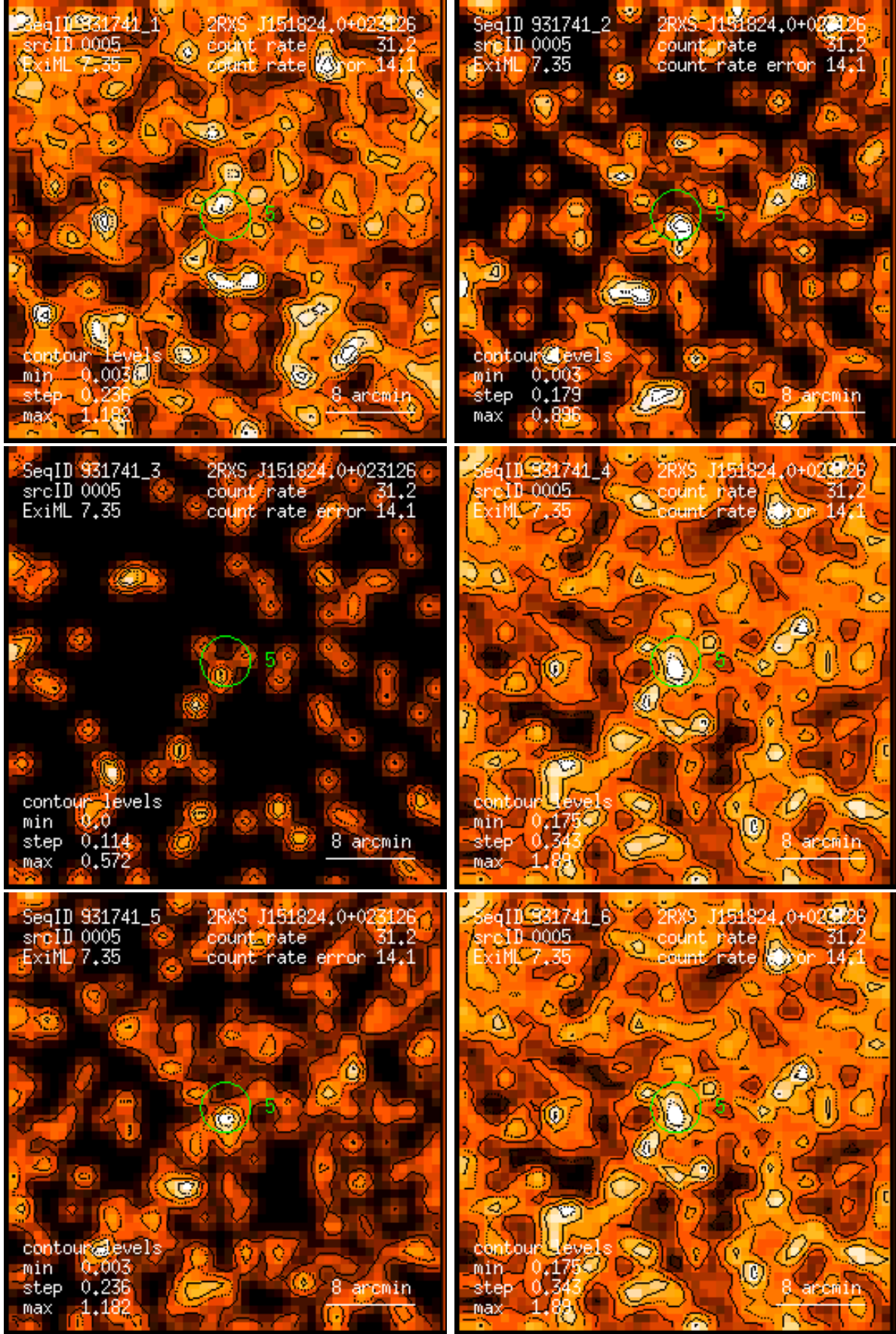
Figure 5: RASS 931741: detection 0005: band rate images, Gaussian filter: (1) PSPC channels 11 – 41, (2) 52 – 90, (3) 91 – 201, (4) 11 – 235, (5) 52 – 201, (6) 11 – 201. Broad band rates in counts/ks. Band rate contour levels in counts/ks/arcmin 2 .
