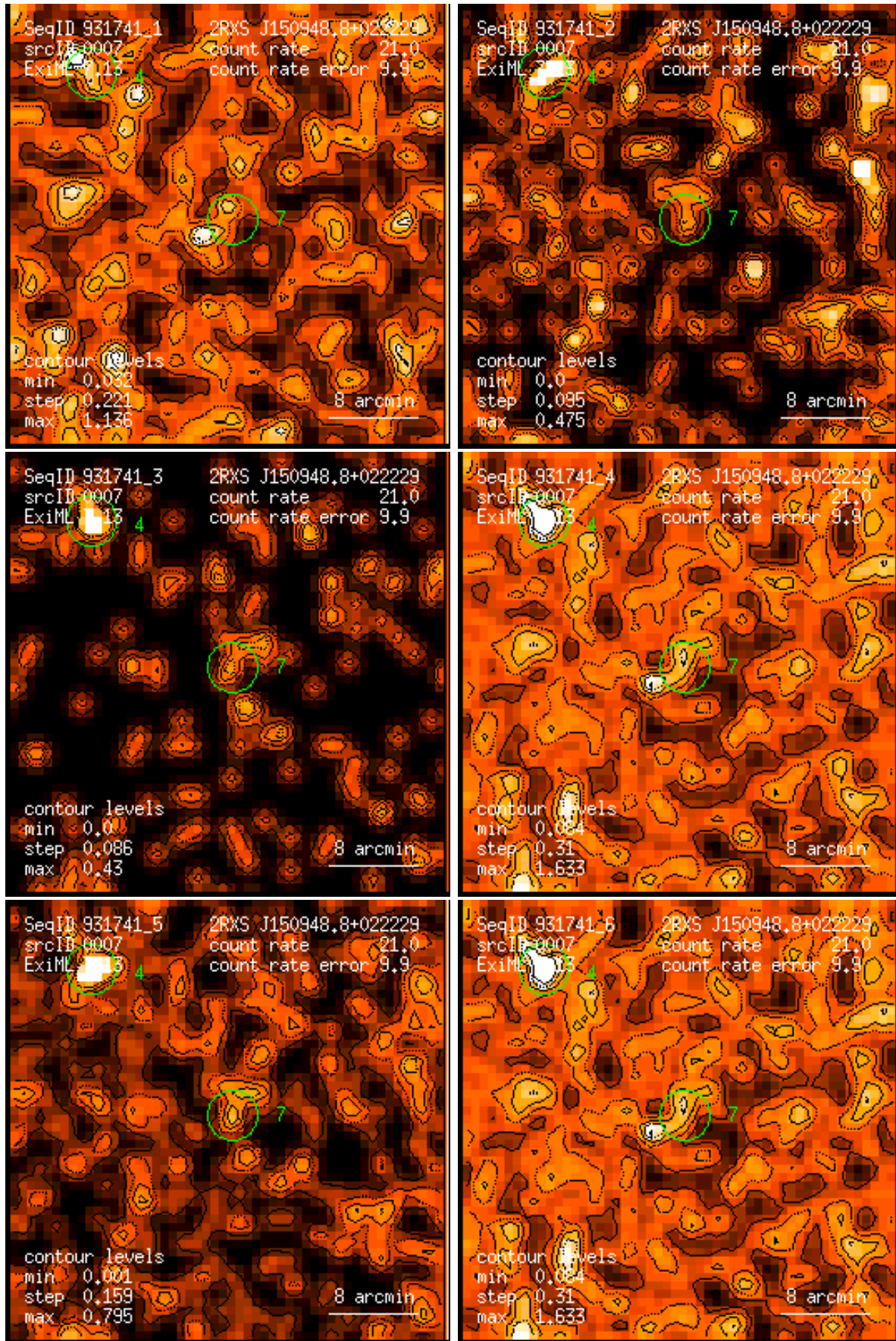
Figure 7: RASS 931741: detection 0007: band rate images, Gaussian filter: (1) PSPC channels 11 – 41, (2) 52 – 90, (3) 91 – 201, (4) 11 – 235, (5) 52 – 201, (6) 11 – 201. Broad band rates in counts/ks. Band rate contour levels in counts/ks/arcmin 2 .
