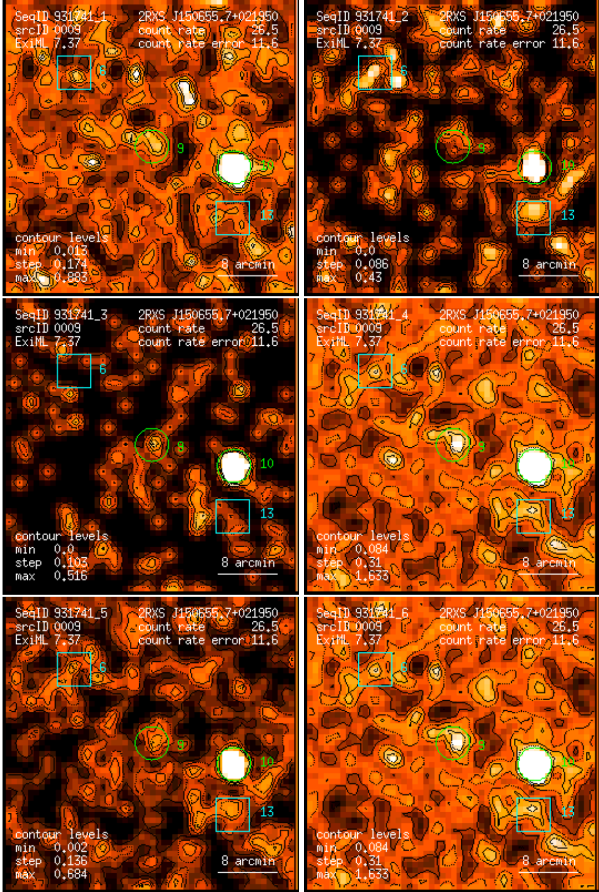
Figure 9: RASS 931741: detection 0009: band rate images, Gaussian filter: (1) PSPC channels 11 – 41, (2) 52 – 90, (3) 91 – 201, (4) 11 – 235, (5) 52 – 201, (6) 11 – 201. Broad band rates in counts/ks. Band rate contour levels in counts/ks/arcmin 2 .
