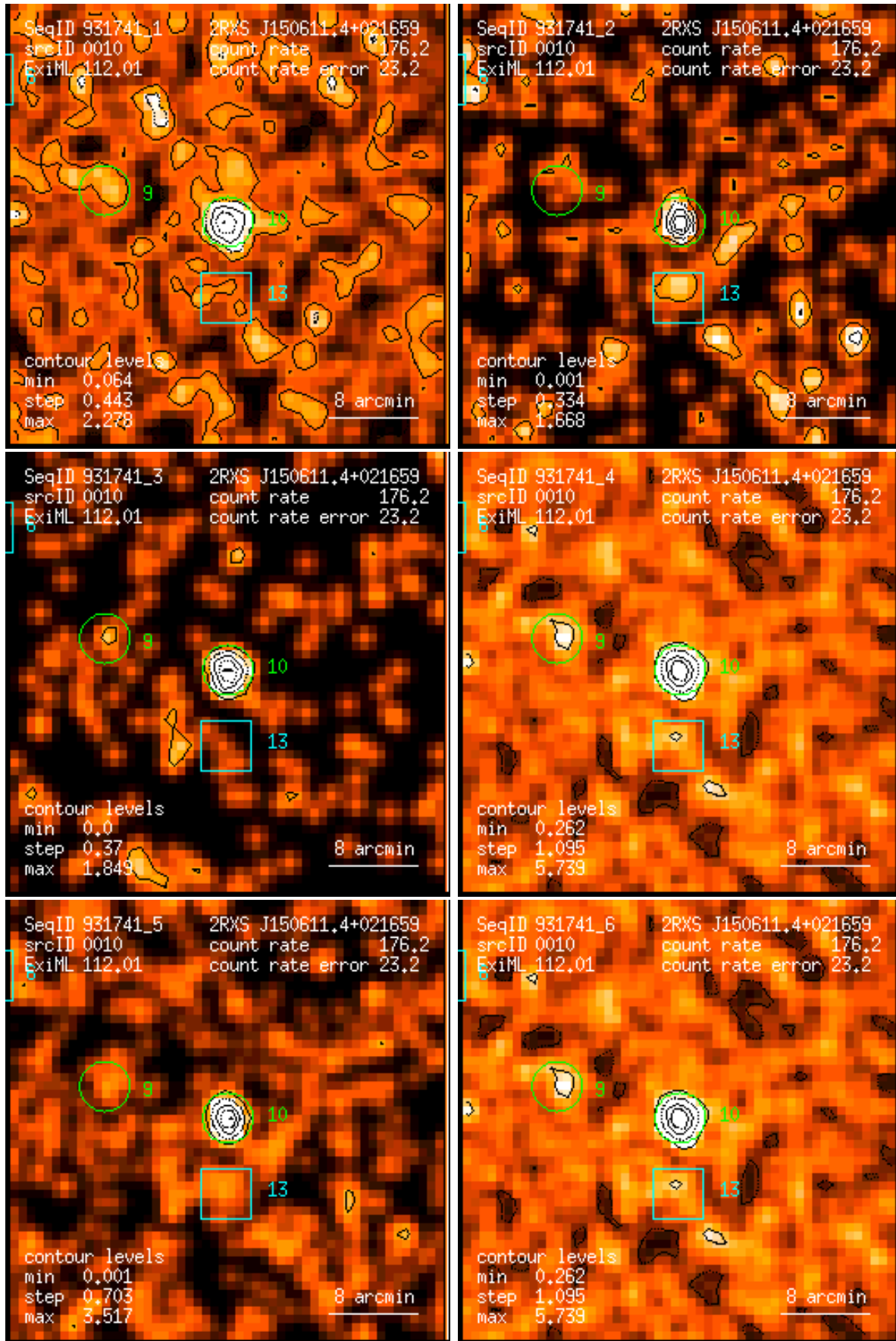
Figure 10: RASS 931741: detection 0010: band rate images, Gaussian filter: (1) PSPC channels 11 – 41, (2) 52 – 90, (3) 91 – 201, (4) 11 – 235, (5) 52 – 201, (6) 11 – 201. Broad band rates in counts/ks. Band rate contour levels in counts/ks/arcmin 2 .
