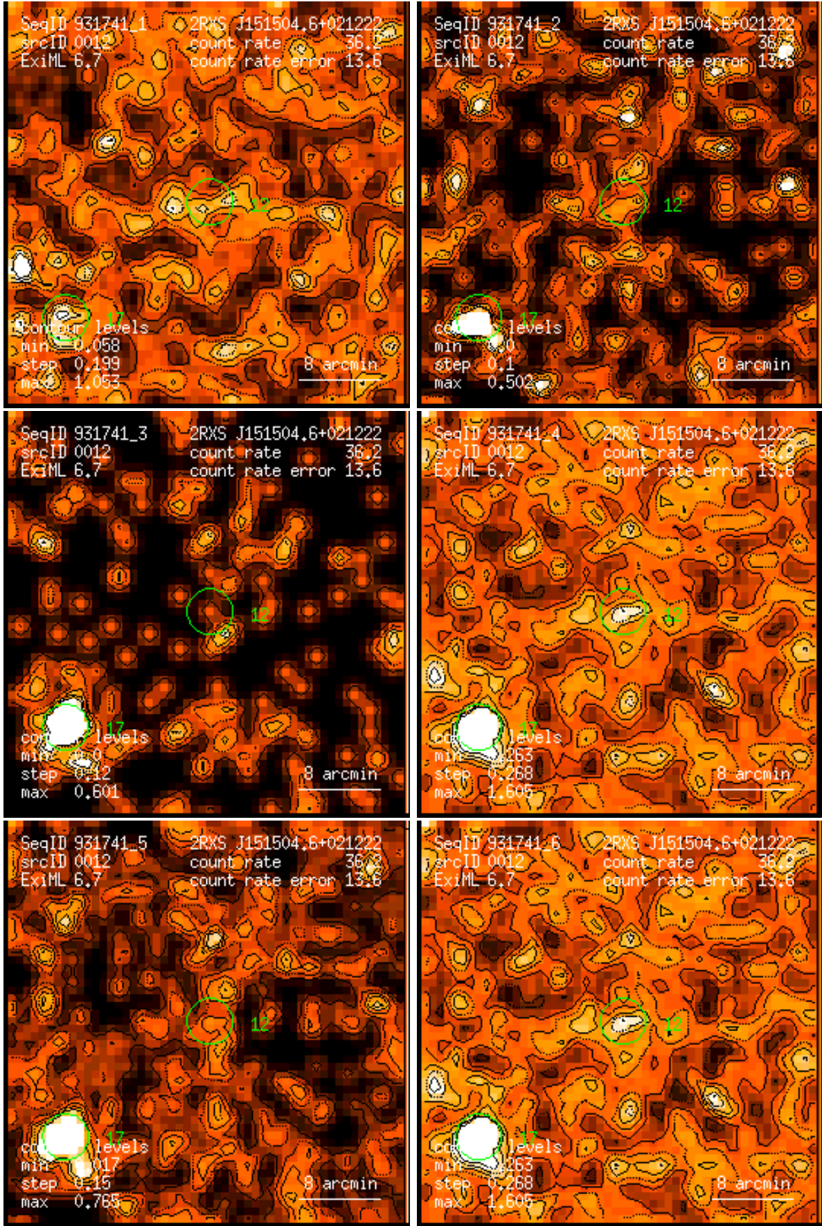
Figure 12: RASS 931741: detection 0012: band rate images, Gaussian filter: (1) PSPC channels 11 – 41, (2) 52 – 90, (3) 91 – 201, (4) 11 – 235, (5) 52 – 201, (6) 11 – 201. Broad band rates in counts/ks. Band rate contour levels in counts/ks/arcmin 2 .
