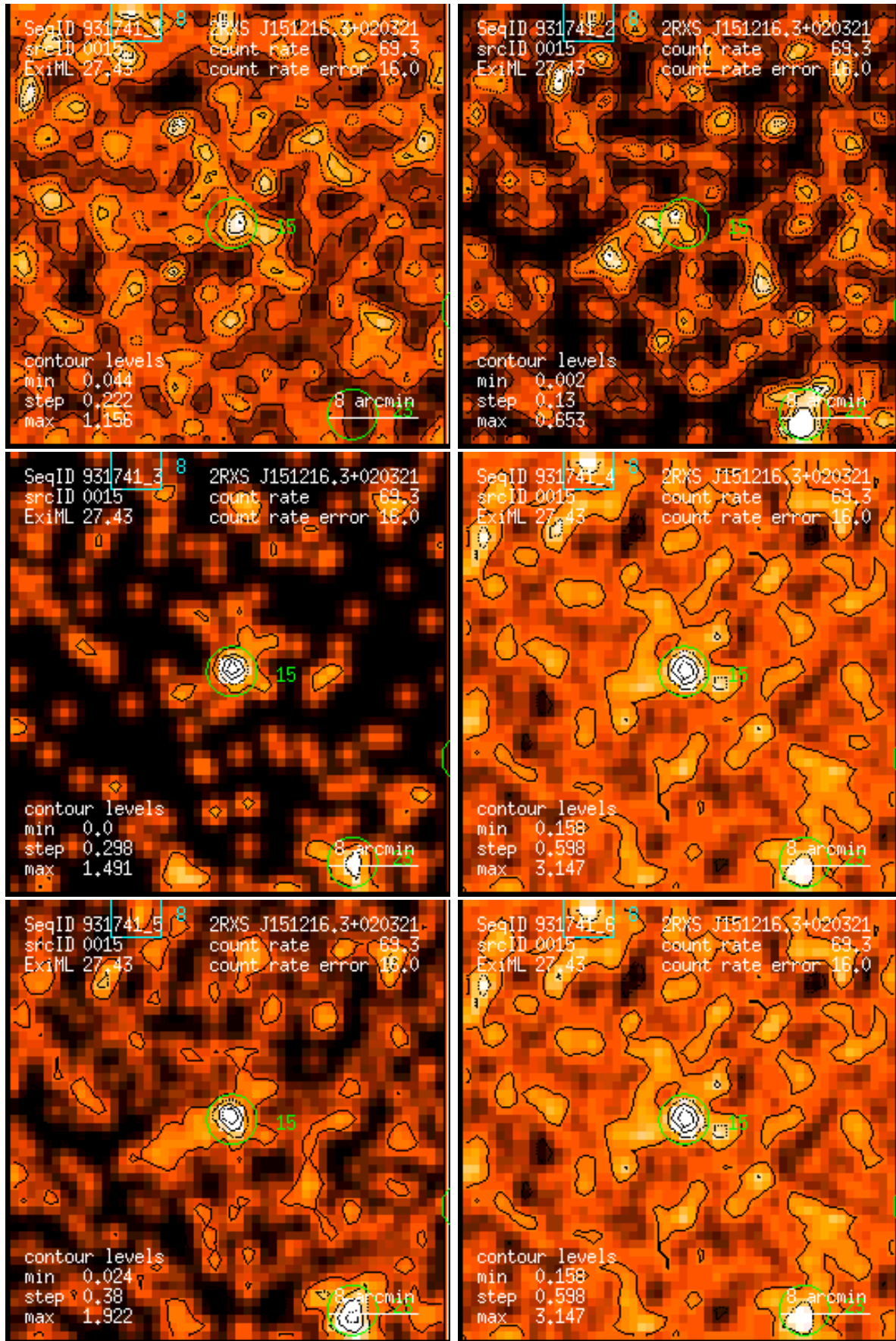
Figure 15: RASS 931741: detection 0015: band rate images, Gaussian filter: (1) PSPC channels 11 – 41, (2) 52 – 90, (3) 91 – 201, (4) 11 – 235, (5) 52 – 201, (6) 11 – 201. Broad band rates in counts/ks. Band rate contour levels in counts/ks/arcmin 2 .
