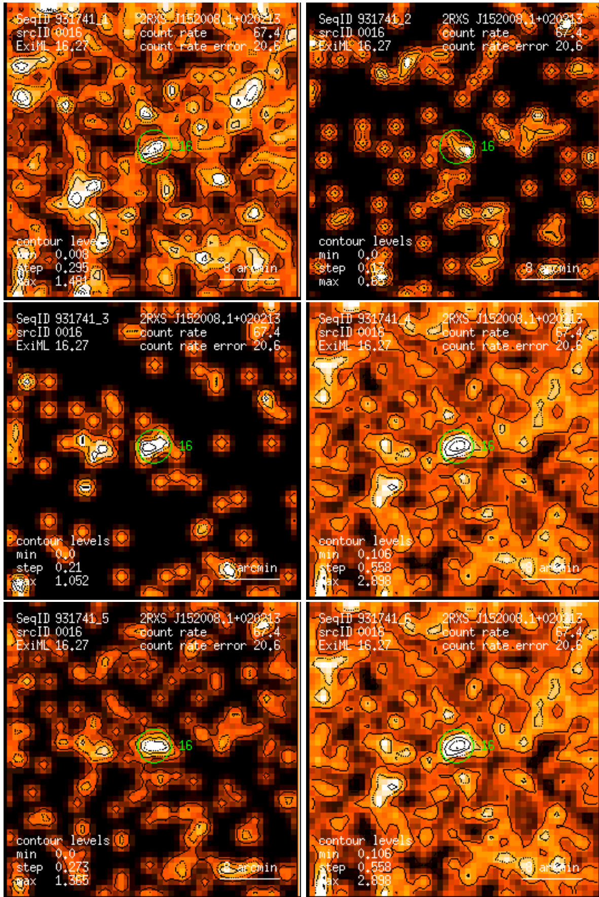
Figure 16: RASS 931741: detection 0016: band rate images, Gaussian filter: (1) PSPC channels 11 – 41, (2) 52 – 90, (3) 91 – 201, (4) 11 – 235, (5) 52 – 201, (6) 11 – 201. Broad band rates in counts/ks. Band rate contour levels in counts/ks/arcmin 2 .
