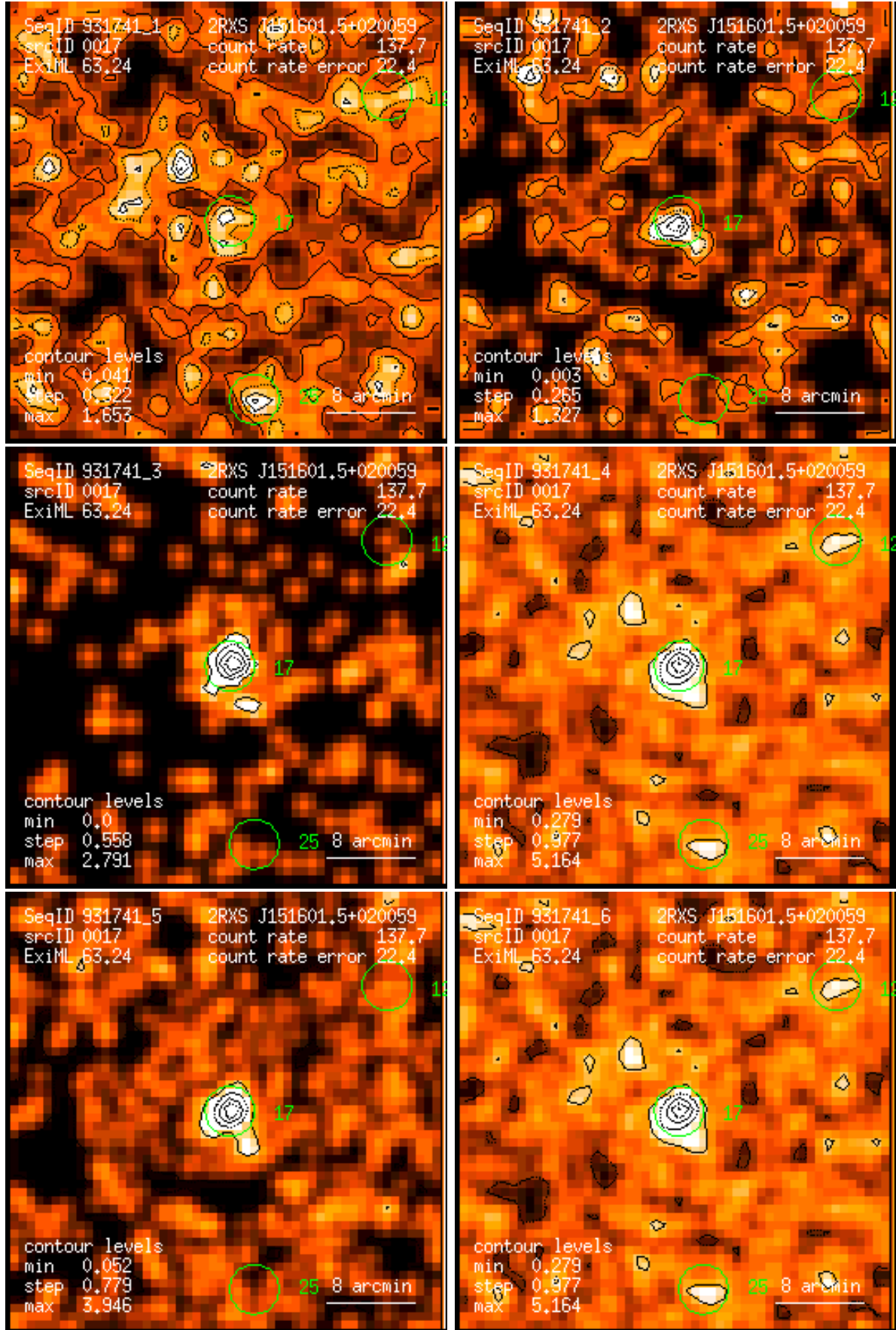
Figure 17: RASS 931741: detection 0017: band rate images, Gaussian filter: (1) PSPC channels 11 – 41, (2) 52 – 90, (3) 91 – 201, (4) 11 – 235, (5) 52 – 201, (6) 11 – 201. Broad band rates in counts/ks. Band rate contour levels in counts/ks/arcmin 2 .
