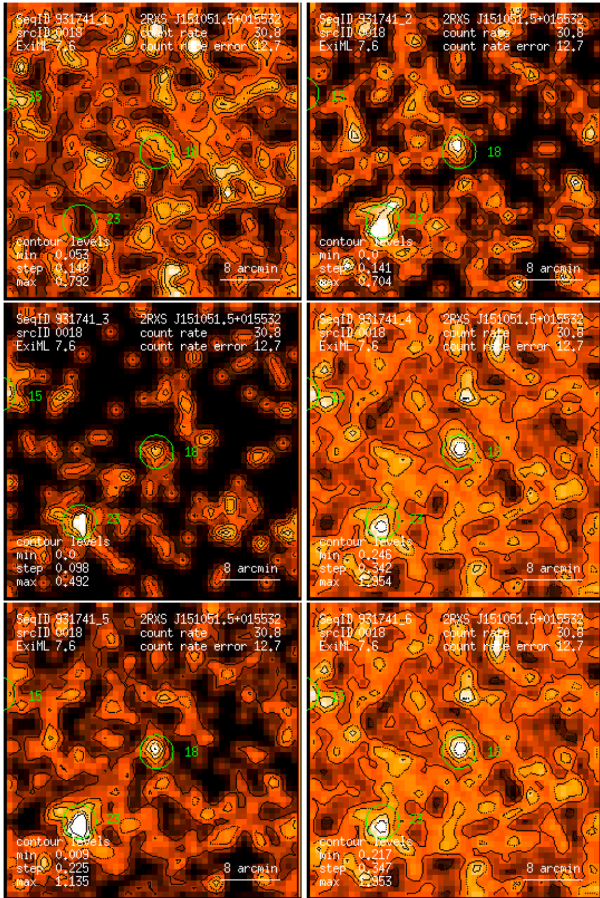
Figure 18: RASS 931741: detection 0018: band rate images, Gaussian filter: (1) PSPC channels 11 – 41, (2) 52 – 90, (3) 91 – 201, (4) 11 – 235, (5) 52 – 201, (6) 11 – 201. Broad band rates in counts/ks. Band rate contour levels in counts/ks/arcmin 2 .
