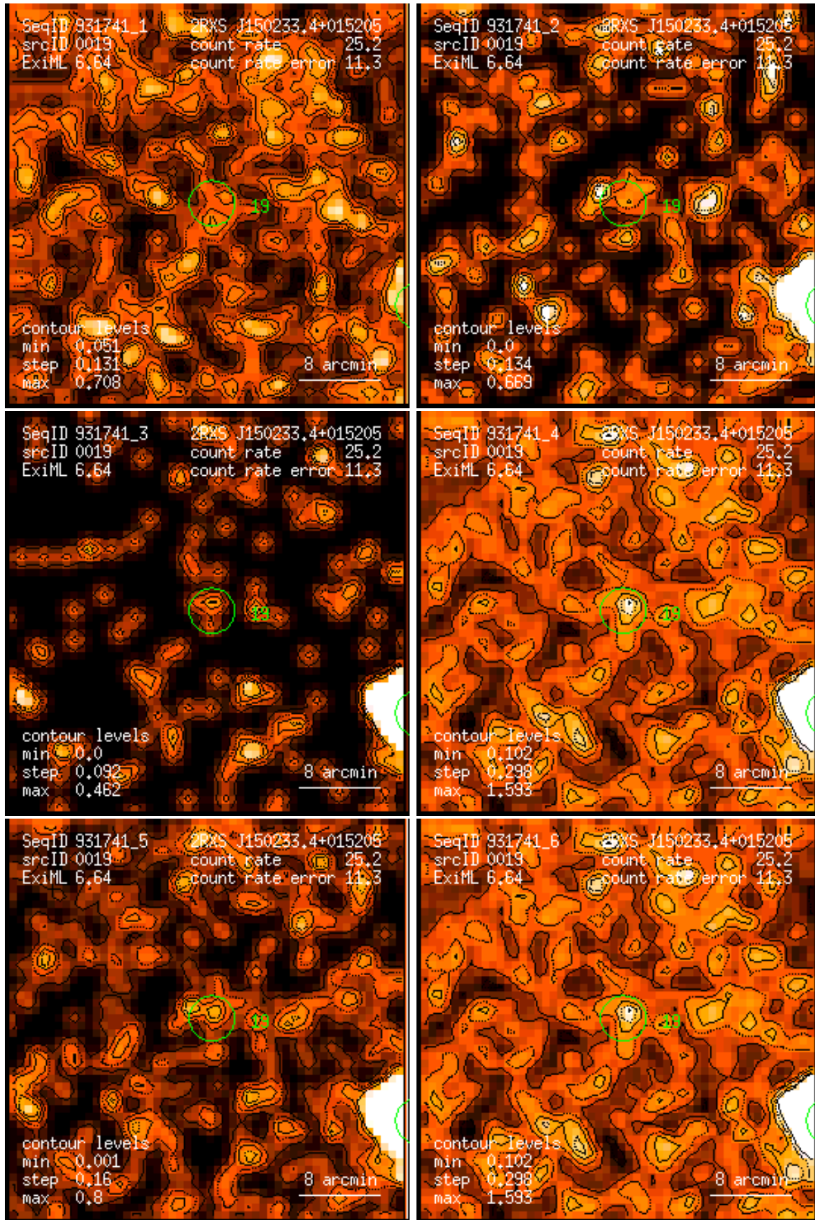
Figure 19: RASS 931741: detection 0019: band rate images, Gaussian filter: (1) PSPC channels 11 – 41, (2) 52 – 90, (3) 91 – 201, (4) 11 – 235, (5) 52 – 201, (6) 11 – 201. Broad band rates in counts/ks. Band rate contour levels in counts/ks/arcmin 2 .
