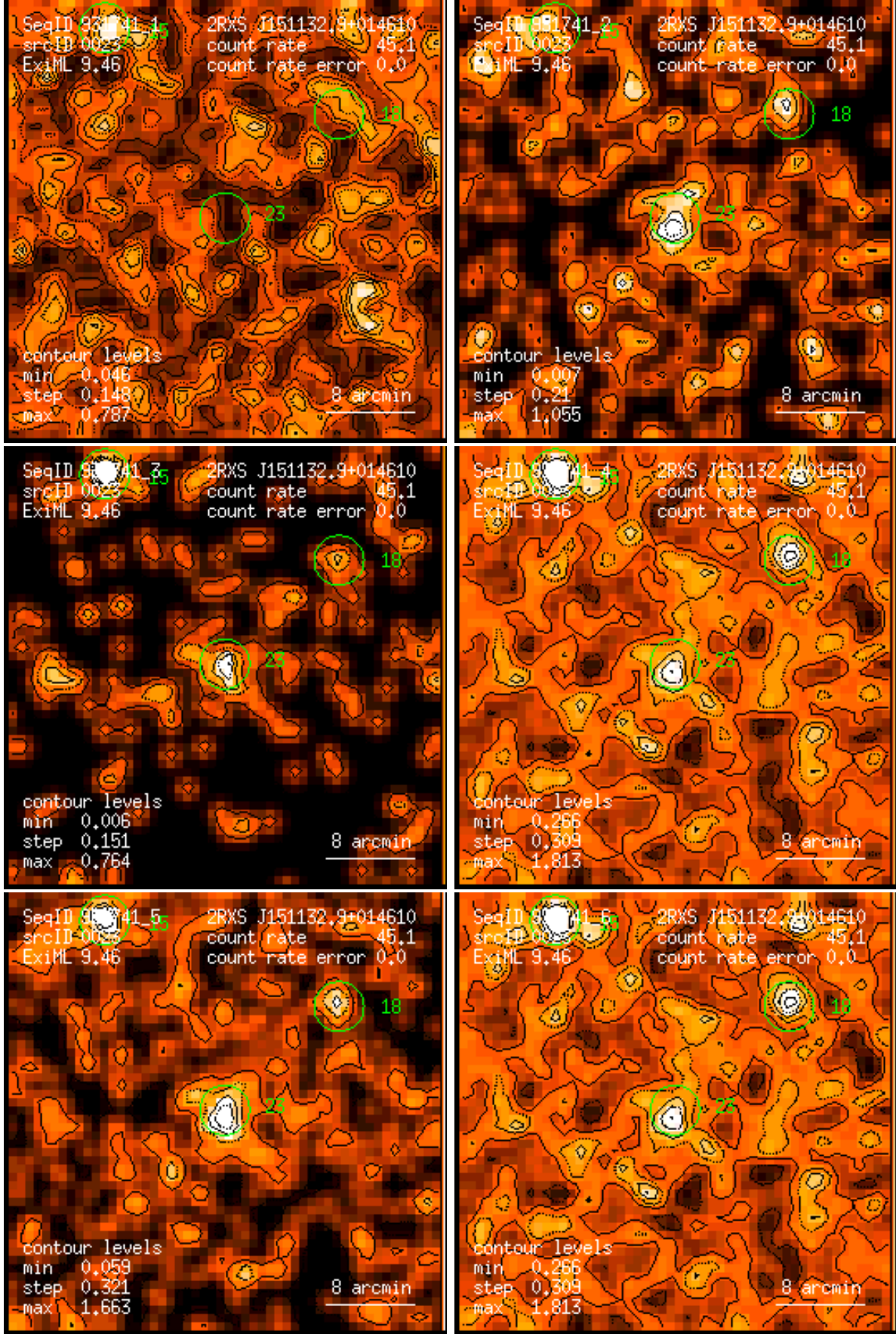
Figure 23: RASS 931741: detection 0023: band rate images, Gaussian filter: (1) PSPC channels 11 – 41, (2) 52 – 90, (3) 91 – 201, (4) 11 – 235, (5) 52 – 201, (6) 11 – 201. Broad band rates in counts/ks. Band rate contour levels in counts/ks/arcmin 2 .
