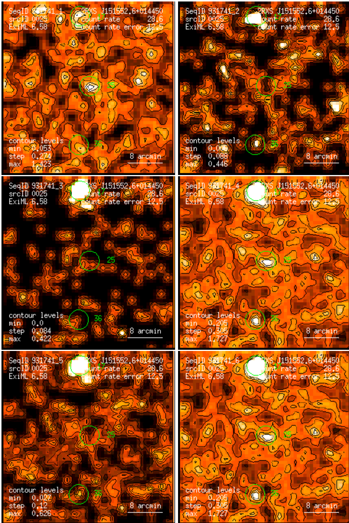
Figure 25: RASS 931741: detection 0025: band rate images, Gaussian filter: (1) PSPC channels 11 – 41, (2) 52 – 90, (3) 91 – 201, (4) 11 – 235, (5) 52 – 201, (6) 11 – 201. Broad band rates in counts/ks. Band rate contour levels in counts/ks/arcmin 2 .
