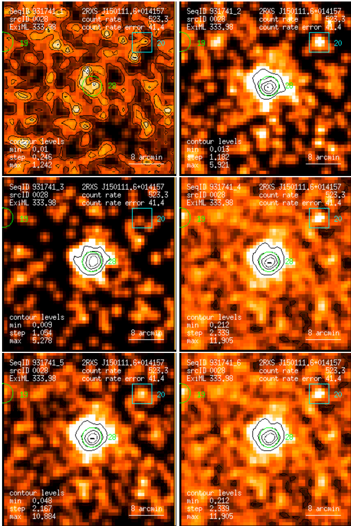
Figure 28: RASS 931741: detection 0028: band rate images, Gaussian filter: (1) PSPC channels 11 – 41, (2) 52 – 90, (3) 91 – 201, (4) 11 – 235, (5) 52 – 201, (6) 11 – 201. Broad band rates in counts/ks. Band rate contour levels in counts/ks/arcmin 2 .
