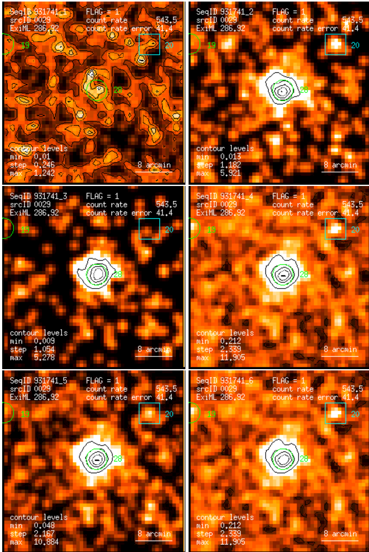
Figure 29: RASS 931741: detection 0029: band rate images, Gaussian filter: (1) PSPC channels 11 – 41, (2) 52 – 90, (3) 91 – 201, (4) 11 – 235, (5) 52 – 201, (6) 11 – 201. Broad band rates in counts/ks. Band rate contour levels in counts/ks/arcmin 2 .
