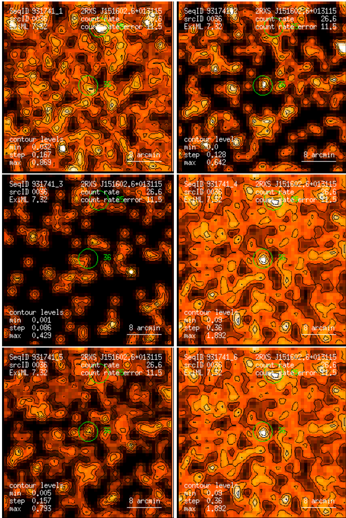
Figure 36: RASS 931741: detection 0036: band rate images, Gaussian filter: (1) PSPC channels 11 – 41, (2) 52 – 90, (3) 91 – 201, (4) 11 – 235, (5) 52 – 201, (6) 11 – 201. Broad band rates in counts/ks. Band rate contour levels in counts/ks/arcmin 2 .
