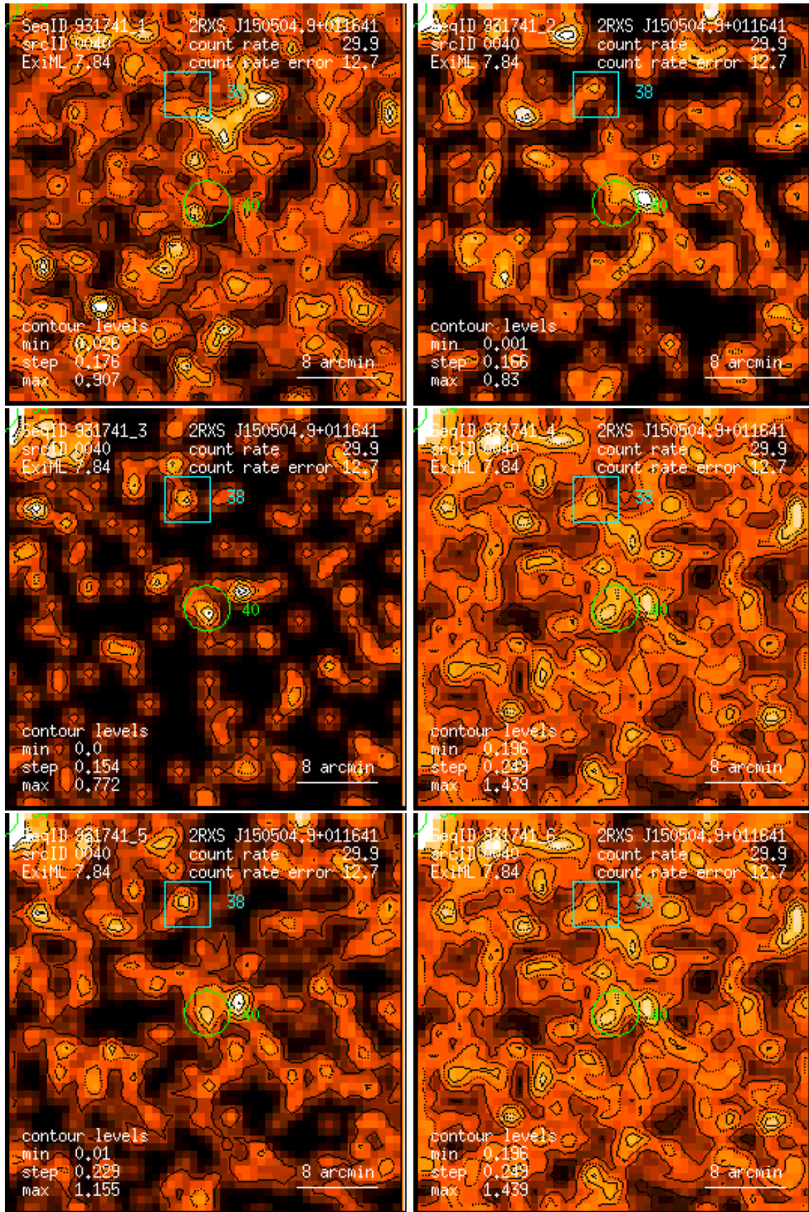
Figure 40: RASS 931741: detection 0040: band rate images, Gaussian filter: (1) PSPC channels 11 – 41, (2) 52 – 90, (3) 91 – 201, (4) 11 – 235, (5) 52 – 201, (6) 11 – 201. Broad band rates in counts/ks. Band rate contour levels in counts/ks/arcmin 2 .
