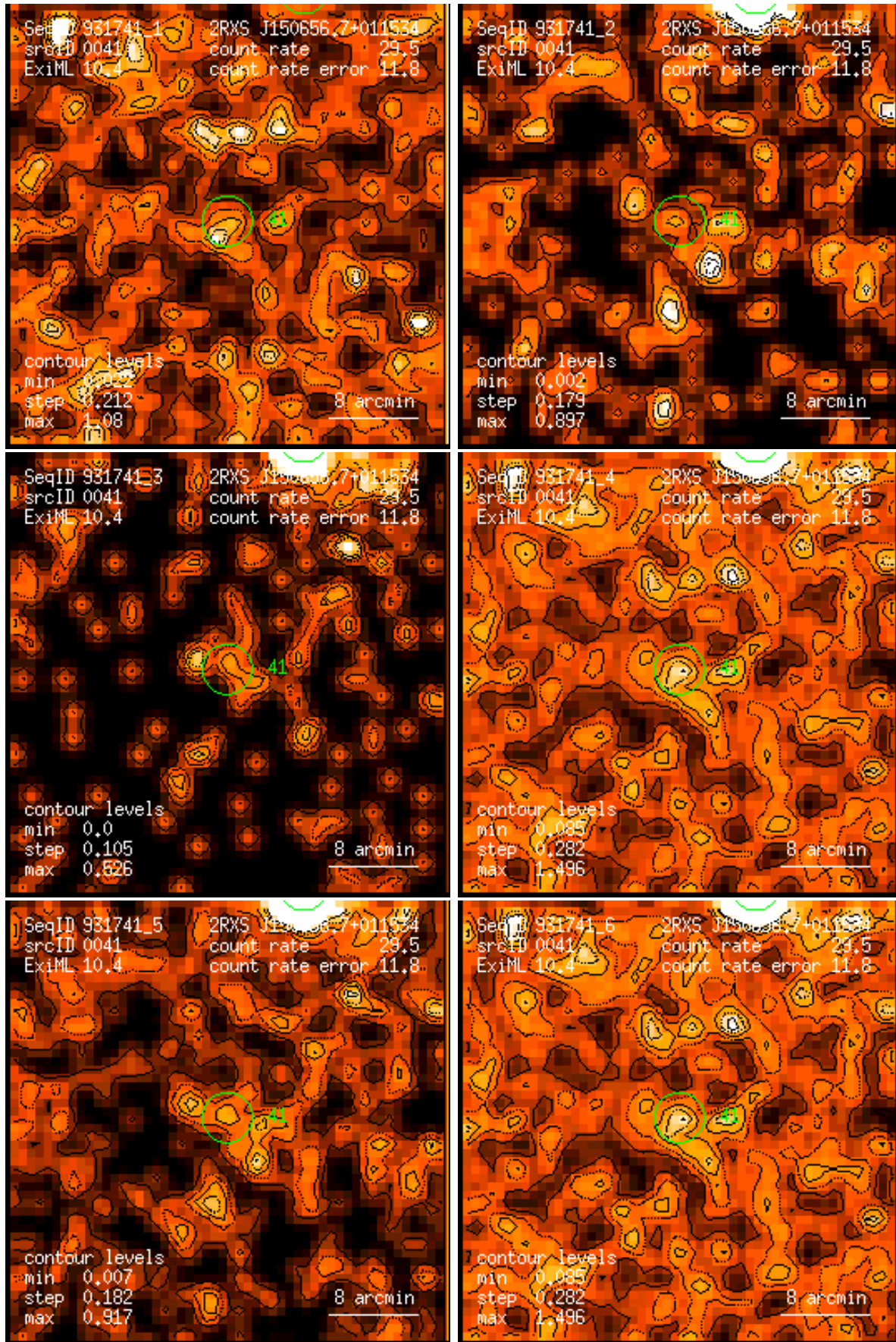
Figure 41: RASS 931741: detection 0041: band rate images, Gaussian filter: (1) PSPC channels 11 – 41, (2) 52 – 90, (3) 91 – 201, (4) 11 – 235, (5) 52 – 201, (6) 11 – 201. Broad band rates in counts/ks. Band rate contour levels in counts/ks/arcmin 2 .
