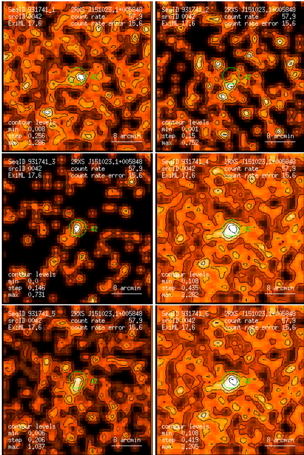
Figure 42: RASS 931741: detection 0042: band rate images, Gaussian filter: (1) PSPC channels 11 – 41, (2) 52 – 90, (3) 91 – 201, (4) 11 – 235, (5) 52 – 201, (6) 11 – 201. Broad band rates in counts/ks. Band rate contour levels in counts/ks/arcmin 2 .
