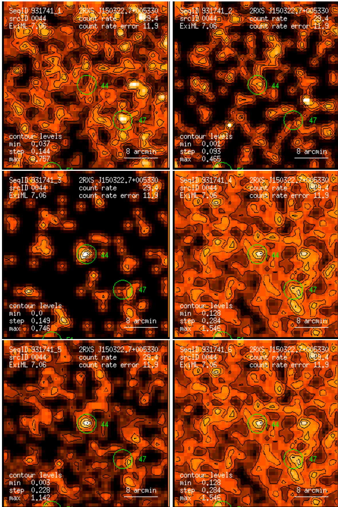
Figure 44: RASS 931741: detection 0044: band rate images, Gaussian filter: (1) PSPC channels 11 – 41, (2) 52 – 90, (3) 91 – 201, (4) 11 – 235, (5) 52 – 201, (6) 11 – 201. Broad band rates in counts/ks. Band rate contour levels in counts/ks/arcmin 2 .
