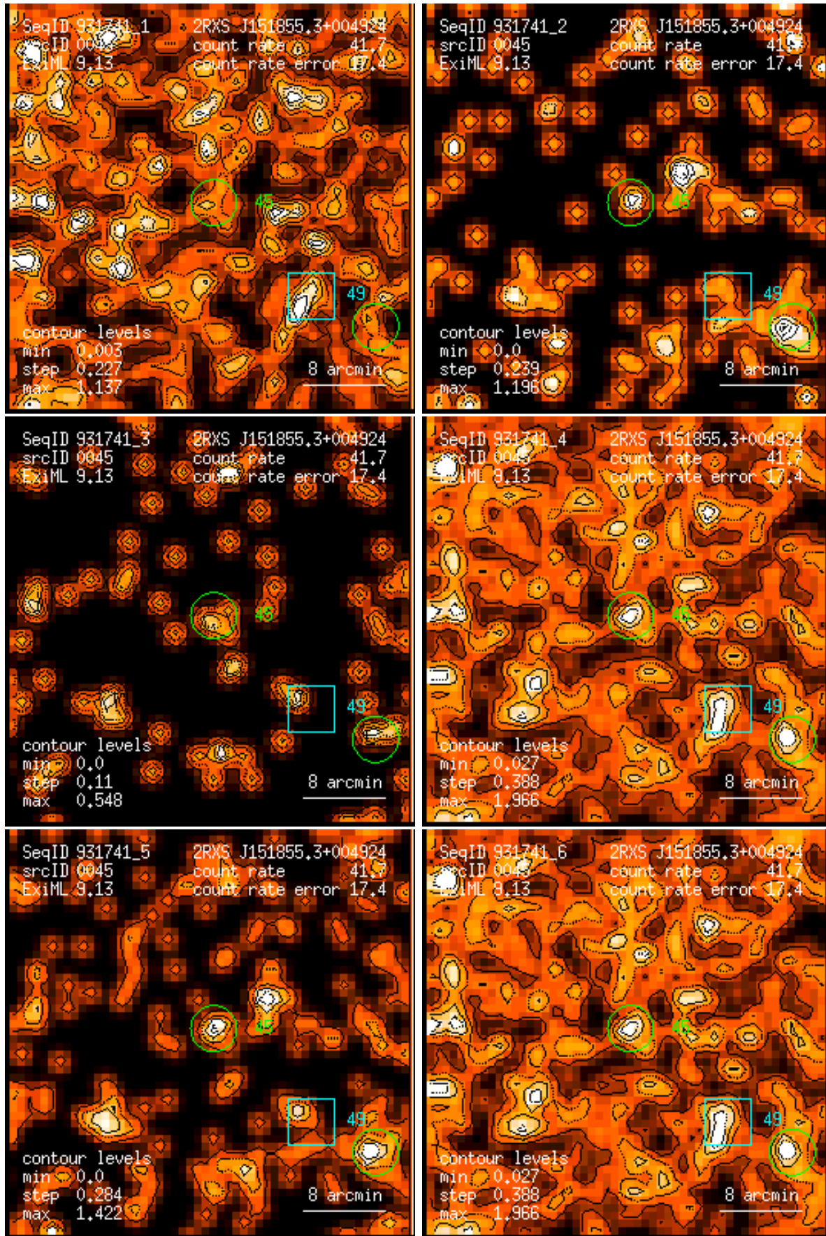
Figure 45: RASS 931741: detection 0045: band rate images, Gaussian filter: (1) PSPC channels 11 – 41, (2) 52 – 90, (3) 91 – 201, (4) 11 – 235, (5) 52 – 201, (6) 11 – 201. Broad band rates in counts/ks. Band rate contour levels in counts/ks/arcmin 2 .
