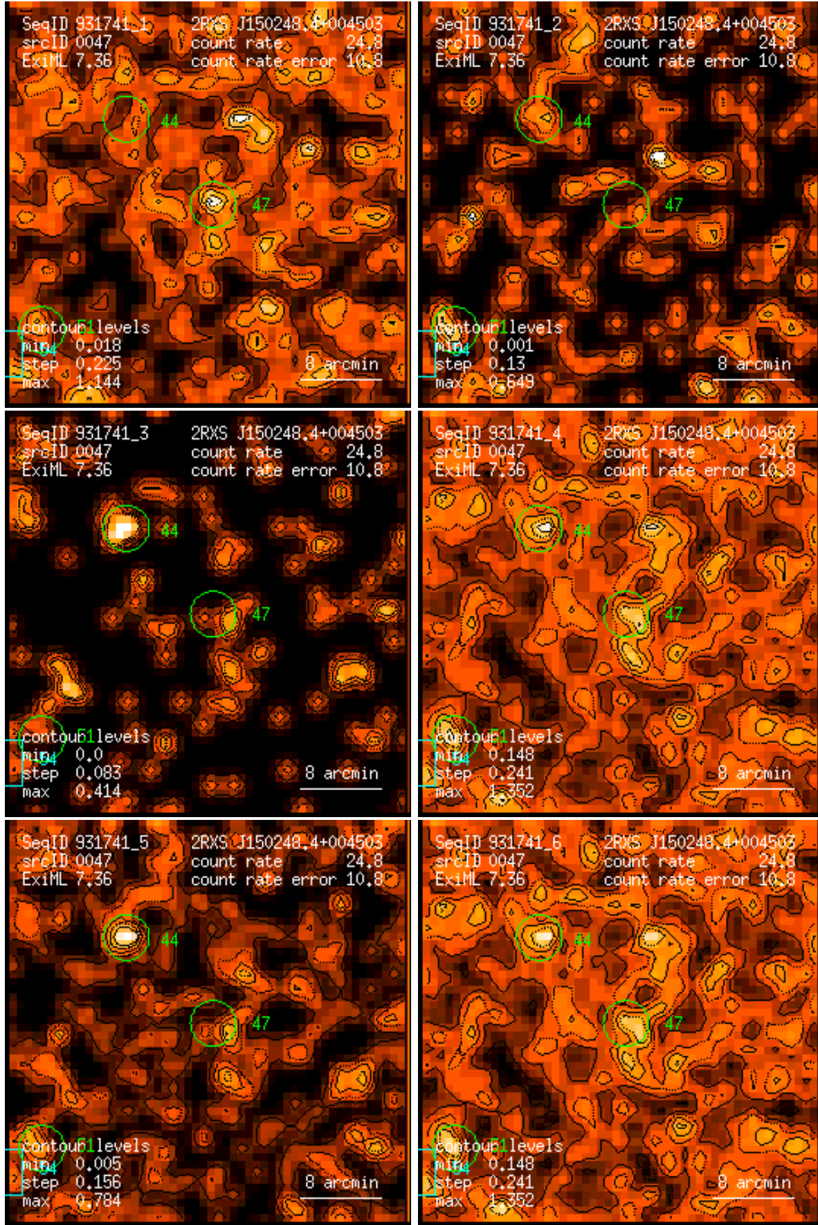
Figure 47: RASS 931741: detection 0047: band rate images, Gaussian filter: (1) PSPC channels 11 – 41, (2) 52 – 90, (3) 91 – 201, (4) 11 – 235, (5) 52 – 201, (6) 11 – 201. Broad band rates in counts/ks. Band rate contour levels in counts/ks/arcmin 2 .
