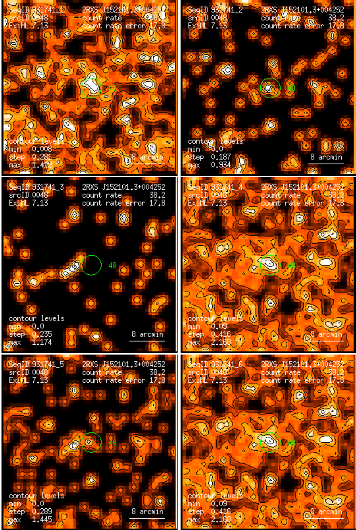
Figure 48: RASS 931741: detection 0048: band rate images, Gaussian filter: (1) PSPC channels 11 – 41, (2) 52 – 90, (3) 91 – 201, (4) 11 – 235, (5) 52 – 201, (6) 11 – 201. Broad band rates in counts/ks. Band rate contour levels in counts/ks/arcmin 2 .
