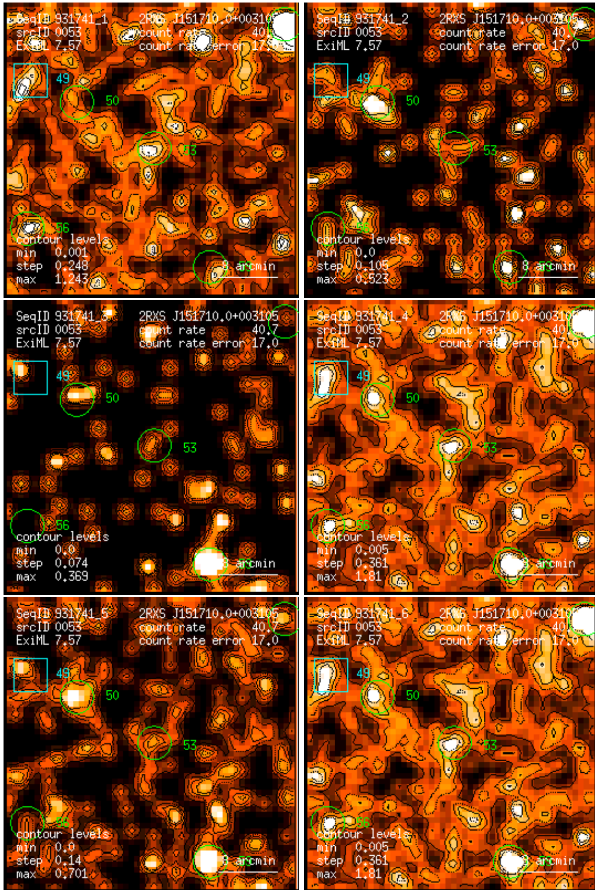
Figure 53: RASS 931741: detection 0053: band rate images, Gaussian filter: (1) PSPC channels 11 – 41, (2) 52 – 90, (3) 91 – 201, (4) 11 – 235, (5) 52 – 201, (6) 11 – 201. Broad band rates in counts/ks. Band rate contour levels in counts/ks/arcmin 2 .
