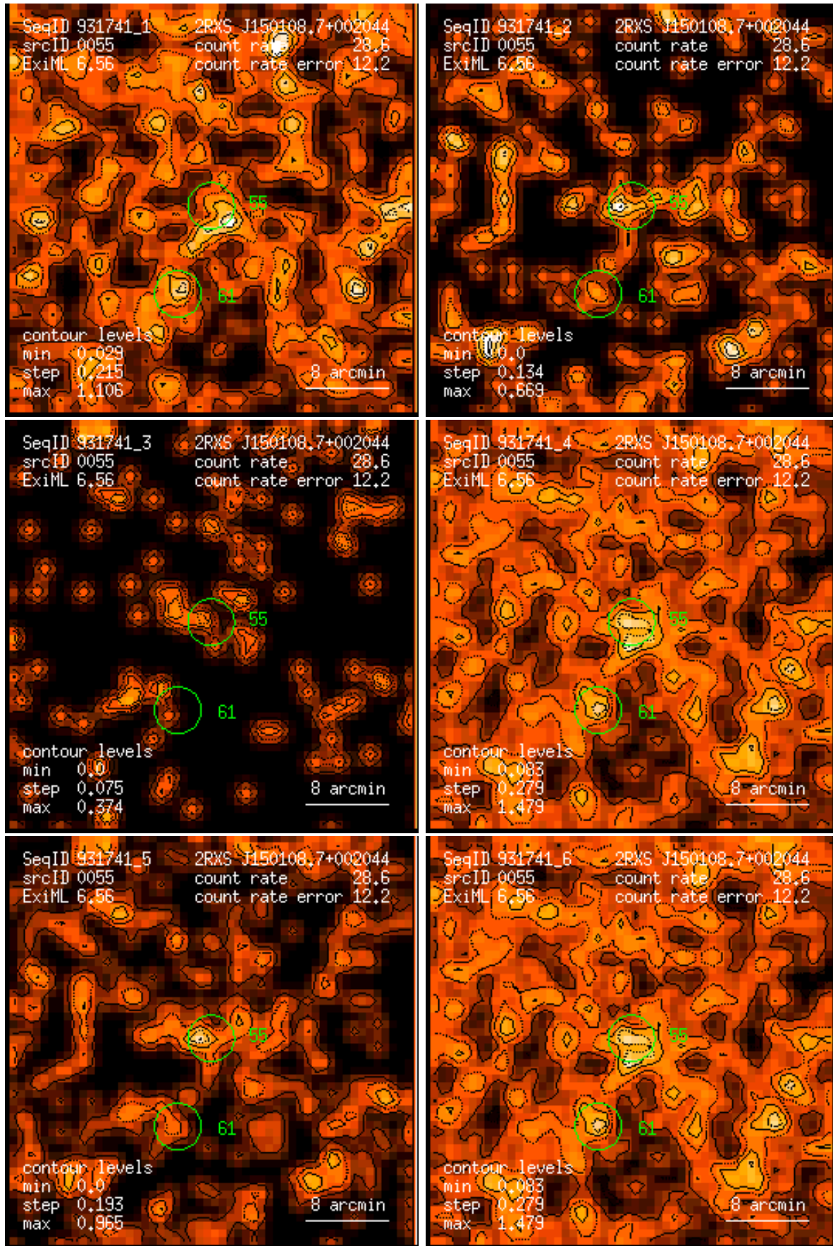
Figure 55: RASS 931741: detection 0055: band rate images, Gaussian filter: (1) PSPC channels 11 – 41, (2) 52 – 90, (3) 91 – 201, (4) 11 – 235, (5) 52 – 201, (6) 11 – 201. Broad band rates in counts/ks. Band rate contour levels in counts/ks/arcmin 2 .
