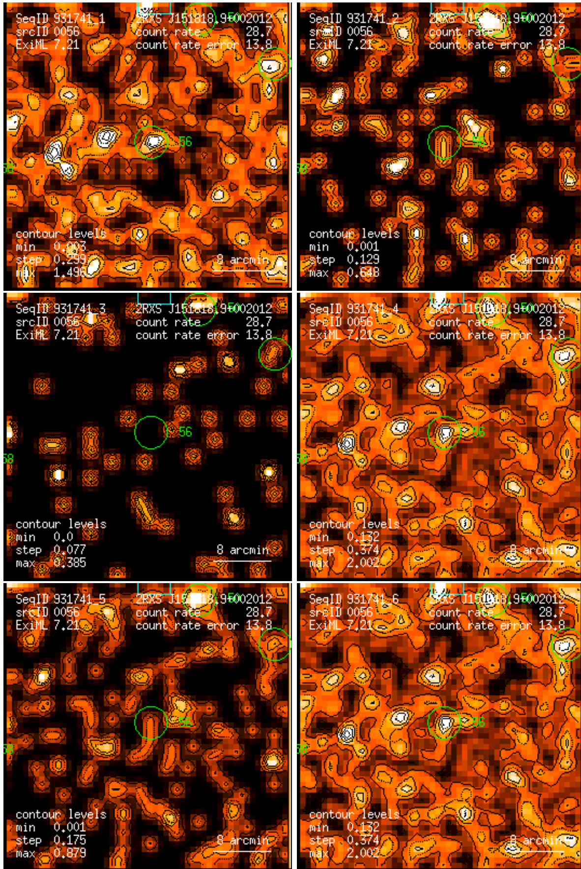
Figure 56: RASS 931741: detection 0056: band rate images, Gaussian filter: (1) PSPC channels 11 – 41, (2) 52 – 90, (3) 91 – 201, (4) 11 – 235, (5) 52 – 201, (6) 11 – 201. Broad band rates in counts/ks. Band rate contour levels in counts/ks/arcmin 2 .
