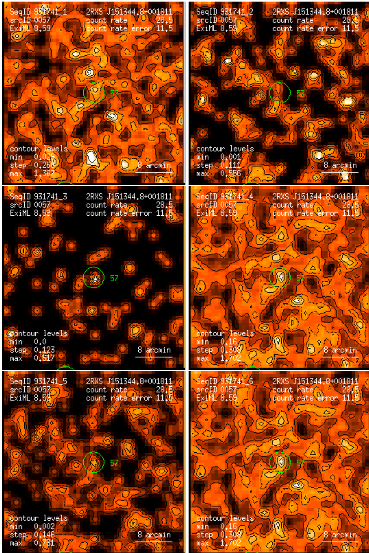
Figure 57: RASS 931741: detection 0057: band rate images, Gaussian filter: (1) PSPC channels 11 – 41, (2) 52 – 90, (3) 91 – 201, (4) 11 – 235, (5) 52 – 201, (6) 11 – 201. Broad band rates in counts/ks. Band rate contour levels in counts/ks/arcmin 2 .
