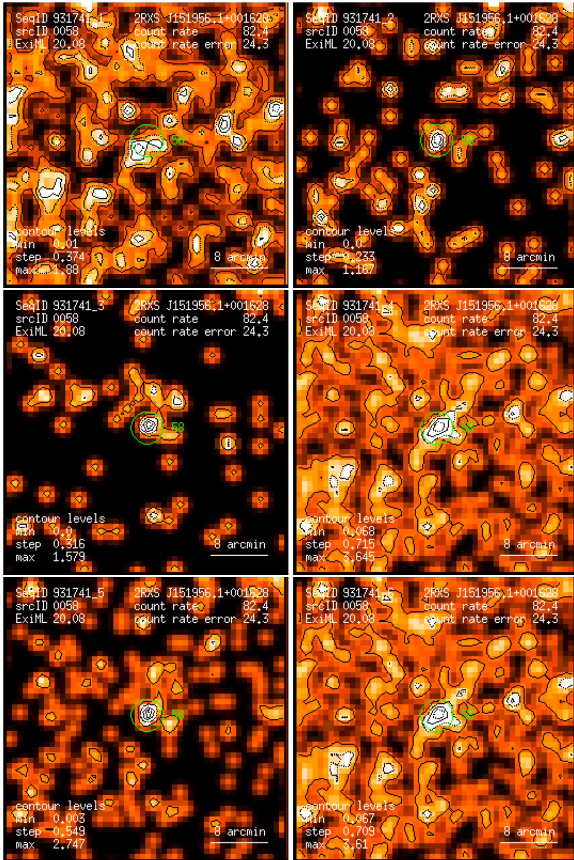
Figure 58: RASS 931741: detection 0058: band rate images, Gaussian filter: (1) PSPC channels 11 – 41, (2) 52 – 90, (3) 91 – 201, (4) 11 – 235, (5) 52 – 201, (6) 11 – 201. Broad band rates in counts/ks. Band rate contour levels in counts/ks/arcmin 2 .
