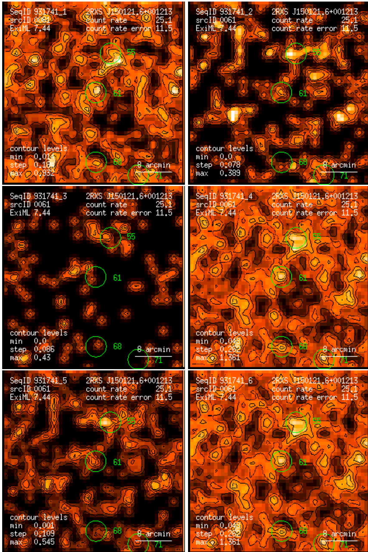
Figure 61: RASS 931741: detection 0061: band rate images, Gaussian filter: (1) PSPC channels 11 – 41, (2) 52 – 90, (3) 91 – 201, (4) 11 – 235, (5) 52 – 201, (6) 11 – 201. Broad band rates in counts/ks. Band rate contour levels in counts/ks/arcmin 2 .
