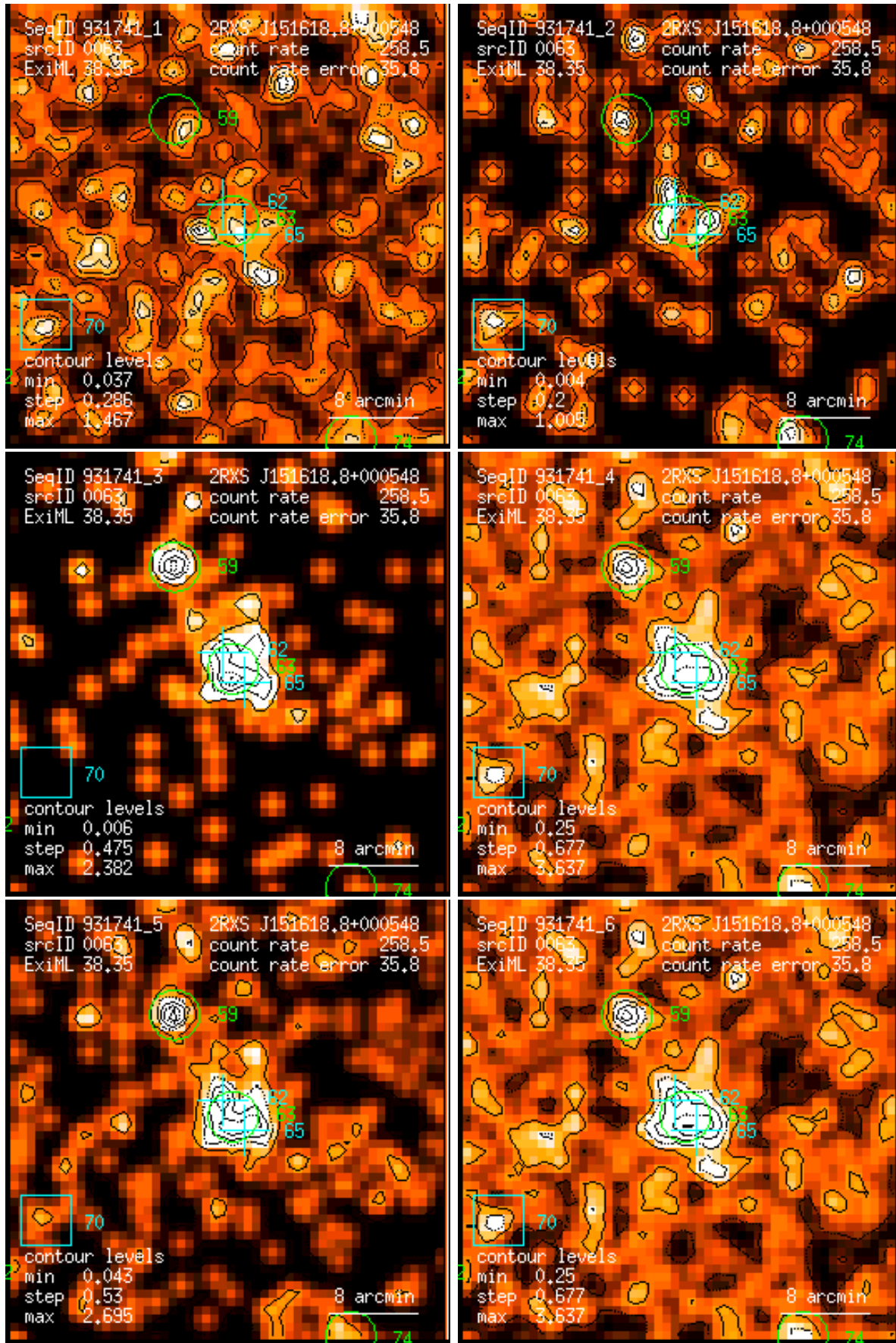
Figure 63: RASS 931741: detection 0063: band rate images, Gaussian filter: (1) PSPC channels 11 – 41, (2) 52 – 90, (3) 91 – 201, (4) 11 – 235, (5) 52 – 201, (6) 11 – 201. Broad band rates in counts/ks. Band rate contour levels in counts/ks/arcmin 2 .
