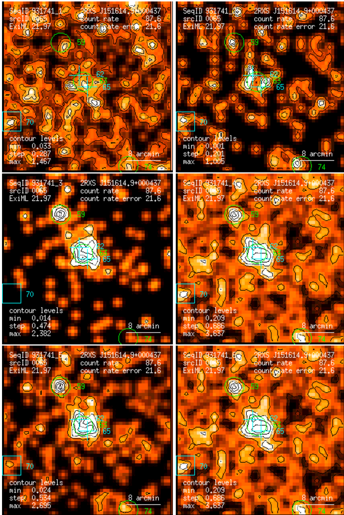
Figure 65: RASS 931741: detection 0065: band rate images, Gaussian filter: (1) PSPC channels 11 – 41, (2) 52 – 90, (3) 91 – 201, (4) 11 – 235, (5) 52 – 201, (6) 11 – 201. Broad band rates in counts/ks. Band rate contour levels in counts/ks/arcmin 2 .
