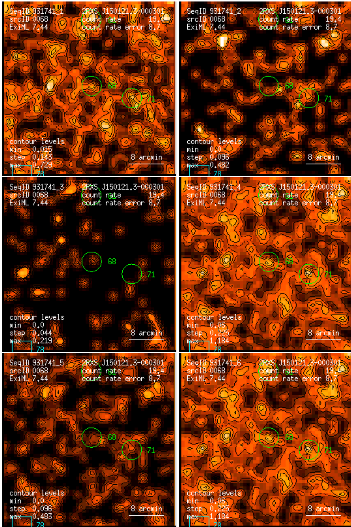
Figure 68: RASS 931741: detection 0068: band rate images, Gaussian filter: (1) PSPC channels 11 – 41, (2) 52 – 90, (3) 91 – 201, (4) 11 – 235, (5) 52 – 201, (6) 11 – 201. Broad band rates in counts/ks. Band rate contour levels in counts/ks/arcmin 2 .
