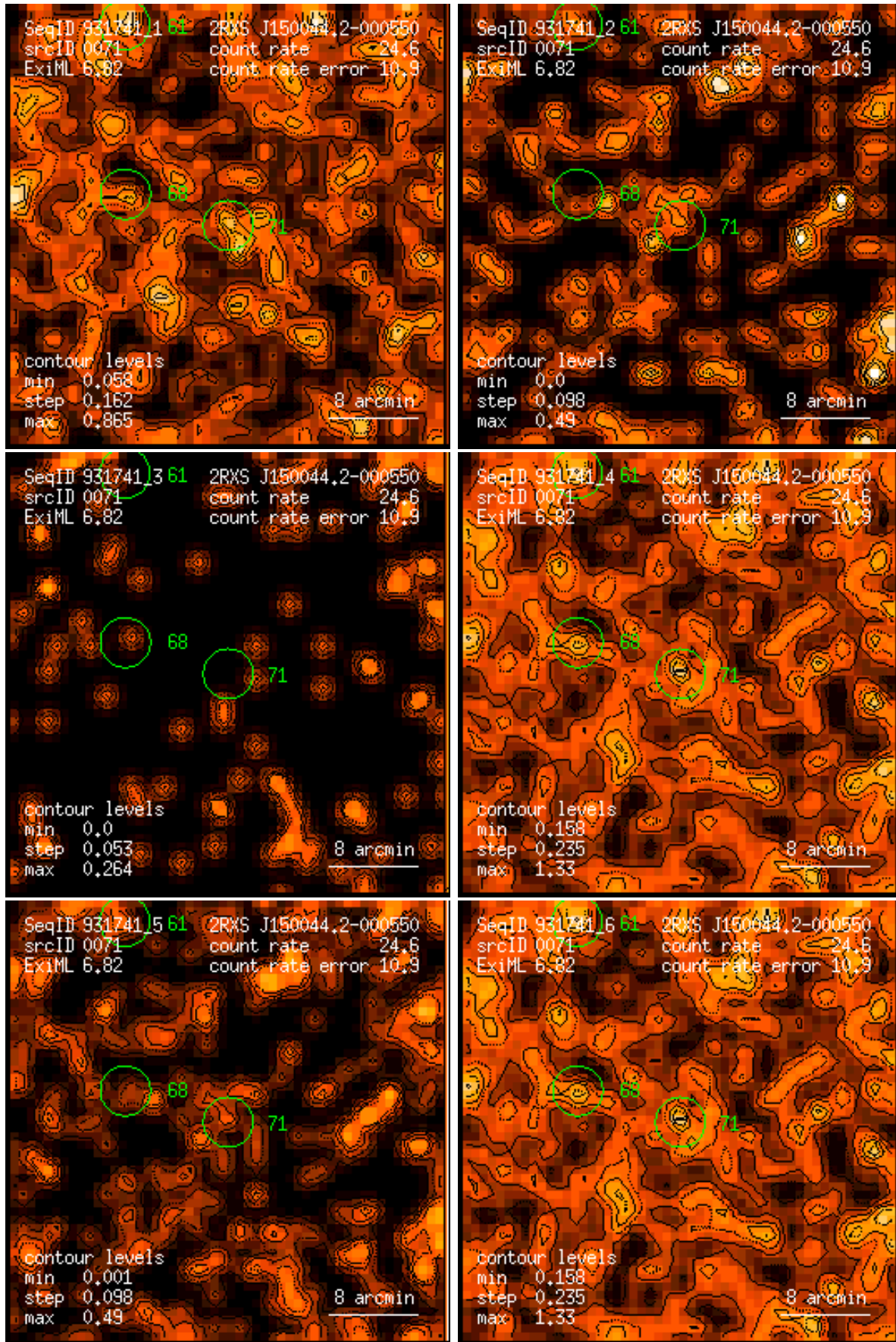
Figure 71: RASS 931741: detection 0071: band rate images, Gaussian filter: (1) PSPC channels 11 – 41, (2) 52 – 90, (3) 91 – 201, (4) 11 – 235, (5) 52 – 201, (6) 11 – 201. Broad band rates in counts/ks. Band rate contour levels in counts/ks/arcmin 2 .
