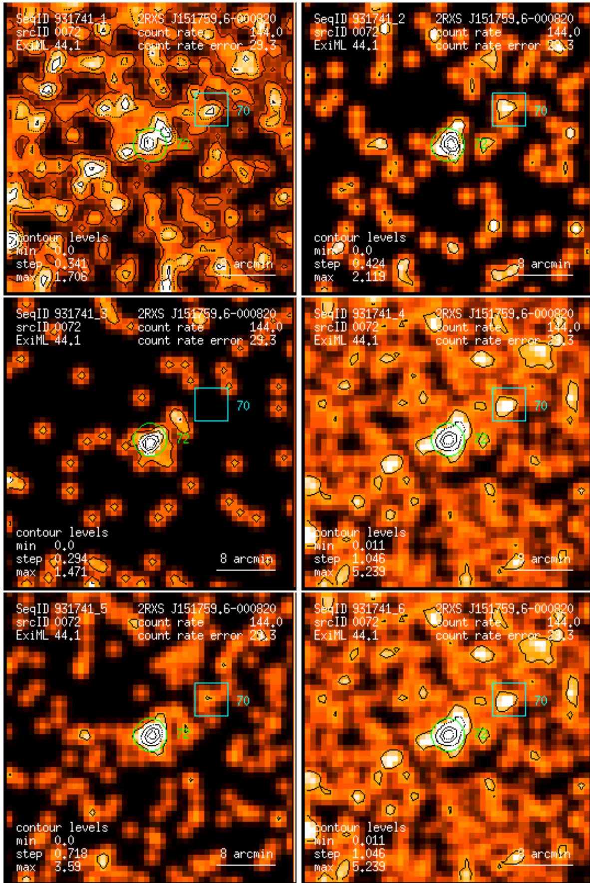
Figure 72: RASS 931741: detection 0072: band rate images, Gaussian filter: (1) PSPC channels 11 – 41, (2) 52 – 90, (3) 91 – 201, (4) 11 – 235, (5) 52 – 201, (6) 11 – 201. Broad band rates in counts/ks. Band rate contour levels in counts/ks/arcmin 2 .
