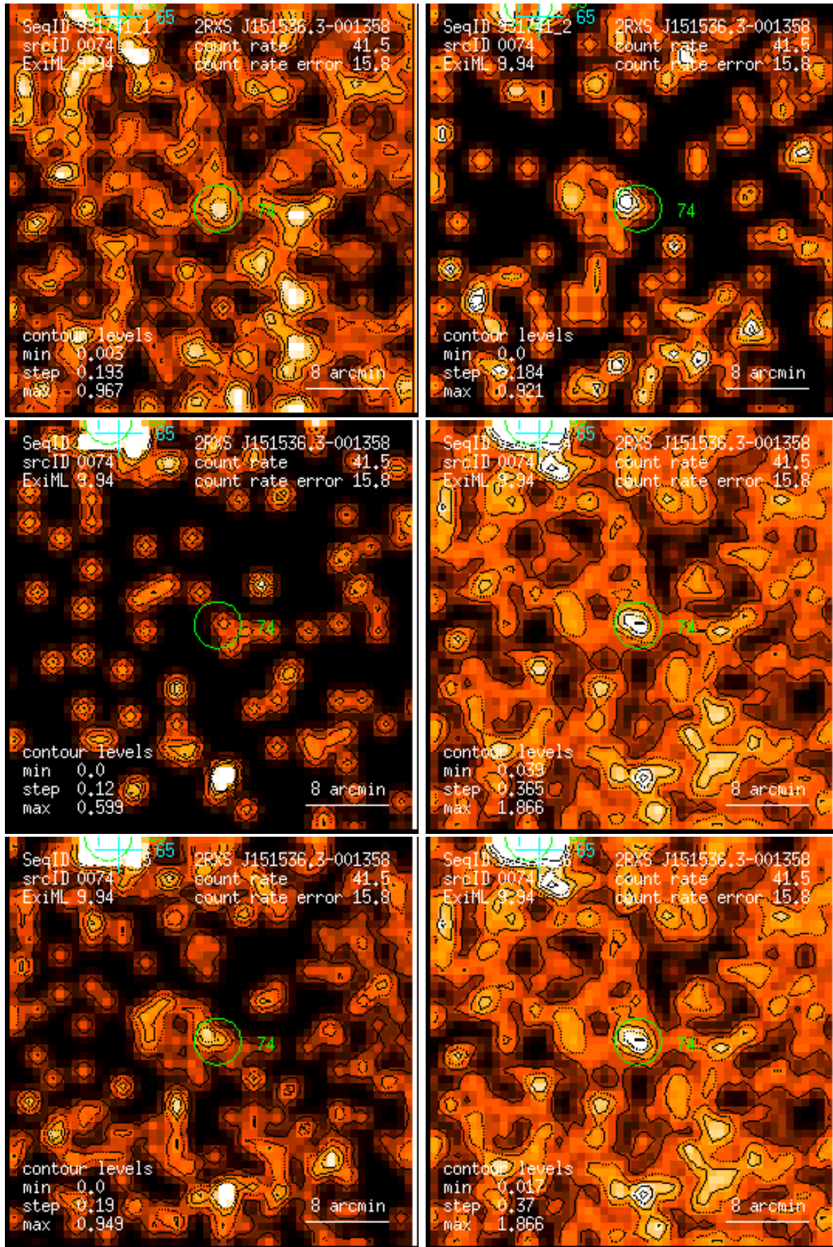
Figure 74: RASS 931741: detection 0074: band rate images, Gaussian filter: (1) PSPC channels 11 – 41, (2) 52 – 90, (3) 91 – 201, (4) 11 – 235, (5) 52 – 201, (6) 11 – 201. Broad band rates in counts/ks. Band rate contour levels in counts/ks/arcmin 2 .
