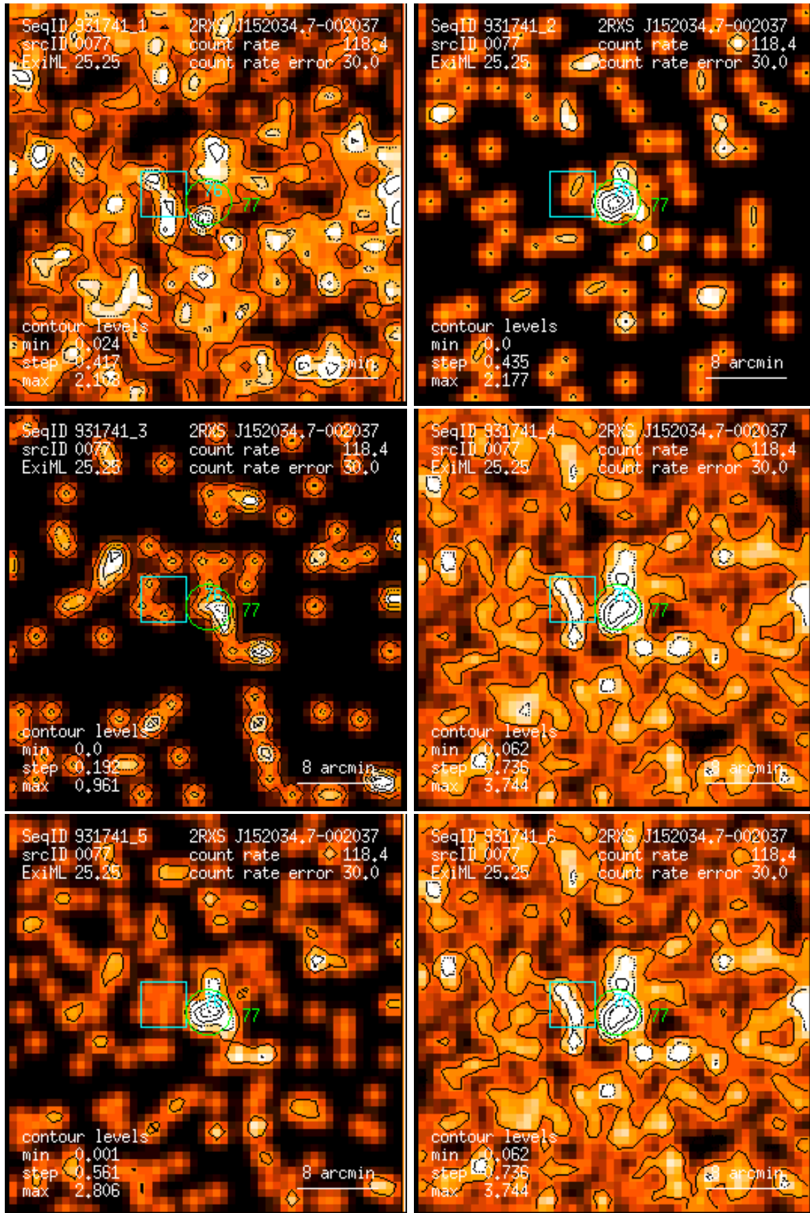
Figure 77: RASS 931741: detection 0077: band rate images, Gaussian filter: (1) PSPC channels 11 – 41, (2) 52 – 90, (3) 91 – 201, (4) 11 – 235, (5) 52 – 201, (6) 11 – 201. Broad band rates in counts/ks. Band rate contour levels in counts/ks/arcmin 2 .
